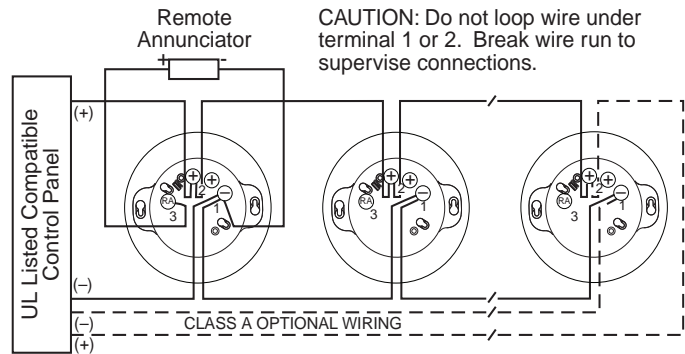
FIGURE 3. TYPICAL WIRING DIAGRAM FOR 2-WIRE LOOP
