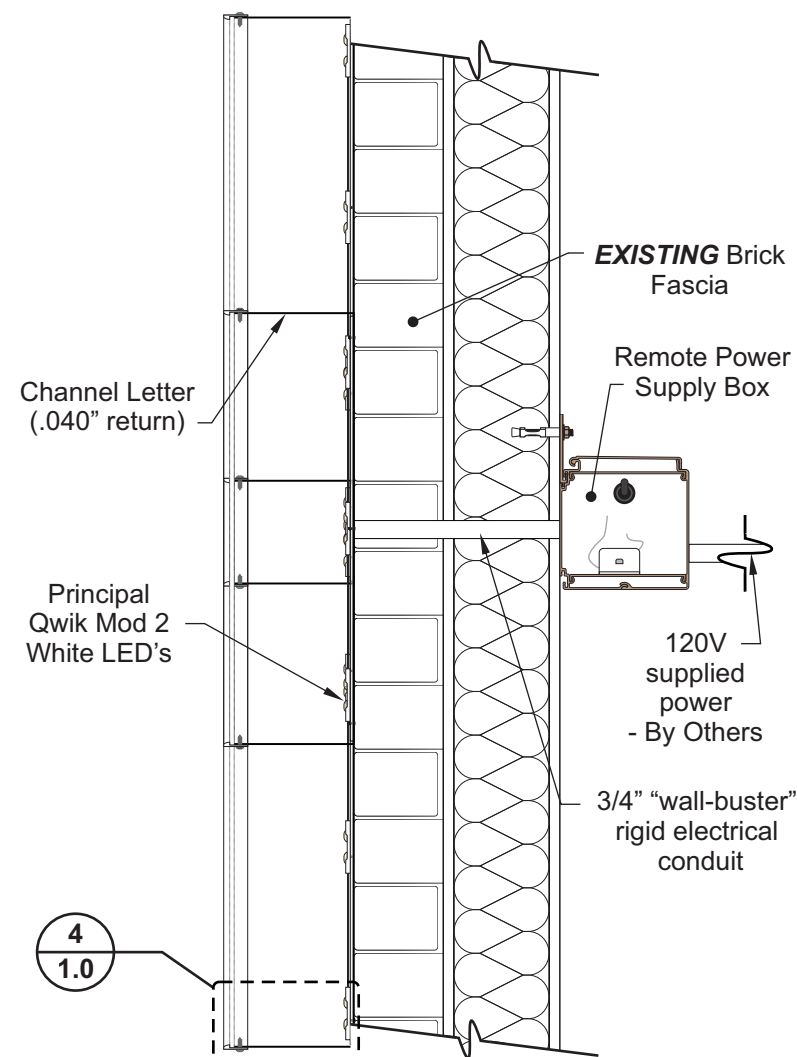
3 ENLARGED END VIEW 1.0 SCALE: 1 1/2" = 1'-0"
