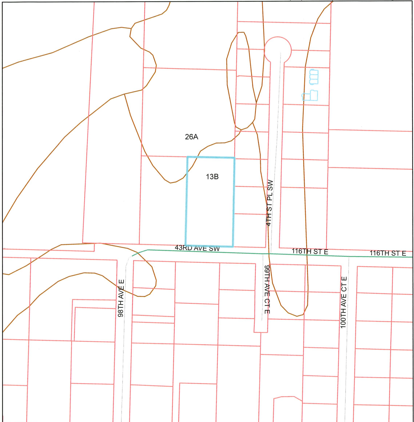
Figure 7 Soils Mapping
