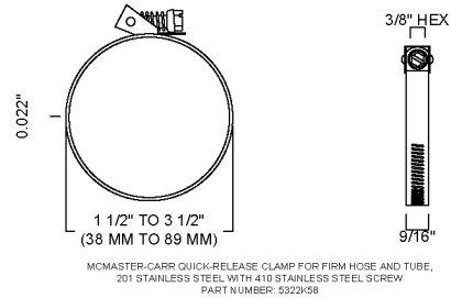
MOUNTING CLAMP
