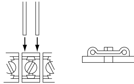
Figure 14: Proper termination
