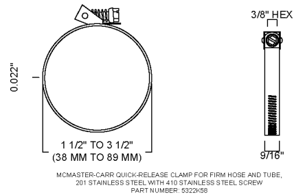
MOUNTING CLAMP
