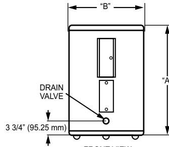
FRONT VIEW DEN 30-120
