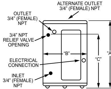
FRONT VIEW DEL 6/10/15/20
