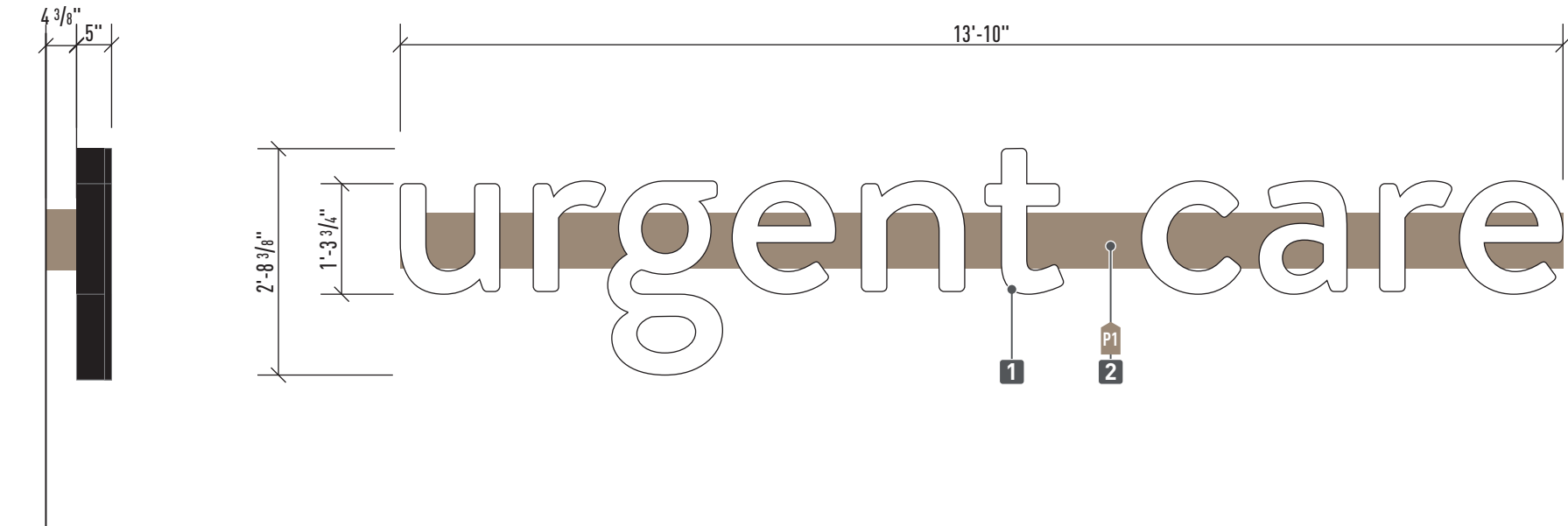
D FACELIT CHANNEL LETTERSET MOUNTED TO RACEWAY QUANTITY: 1 SET MANUFACTURE & INSTALL 37.32 SQ FT SCALE: 1/2" = 1'-0"
