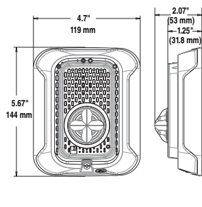
Strobes, Horn Strobes for Walls
