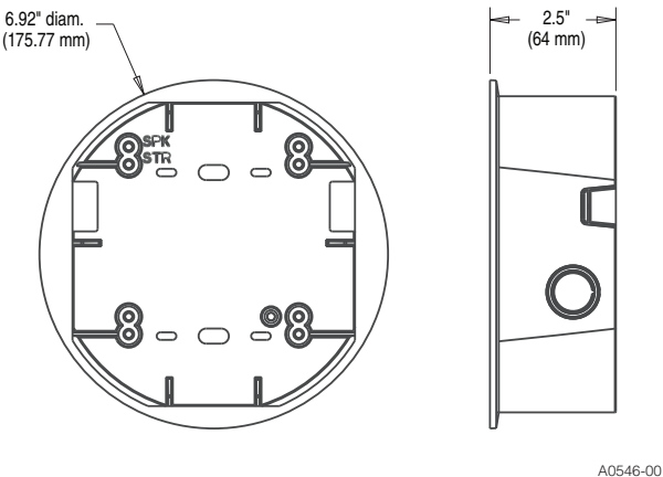
Surface Mount Back Box for Ceilings (SBBCRL, SBCWL)
