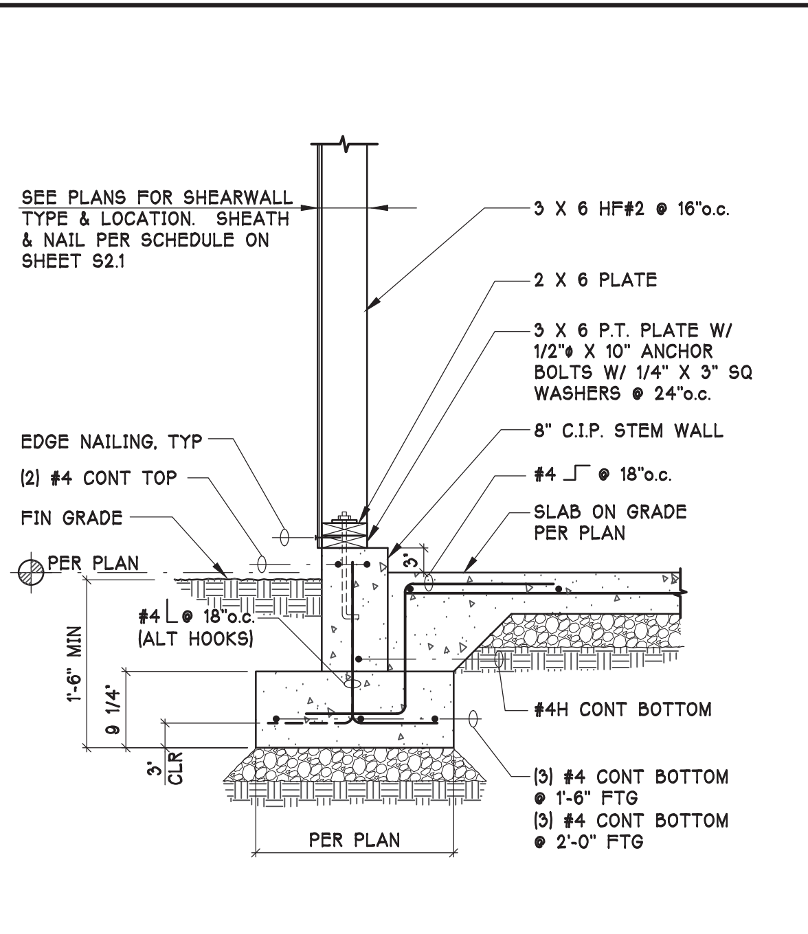
A SECTION 3/4" = 1'-0"
