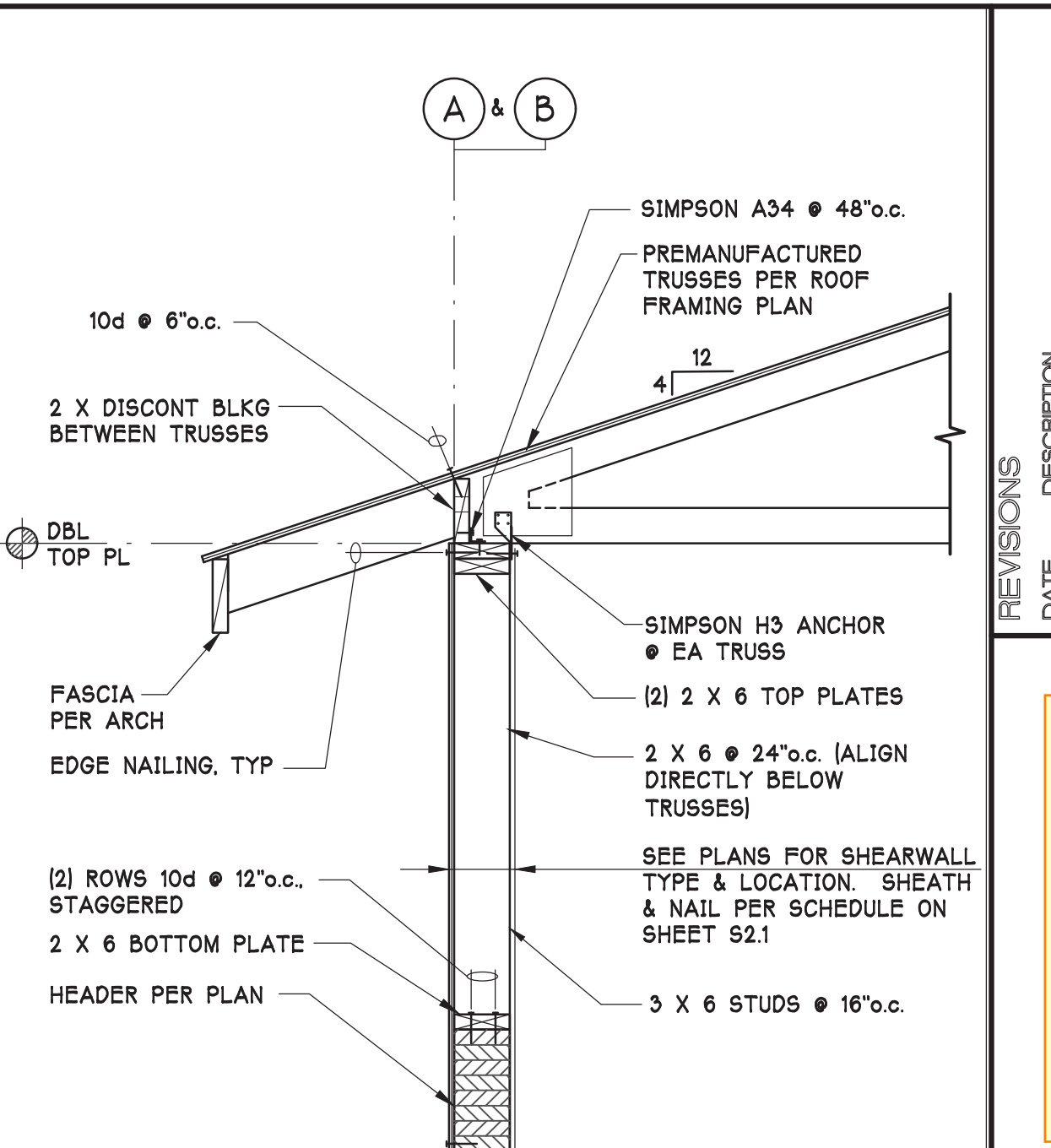
E SECTION 3/4" = 1'-0"
