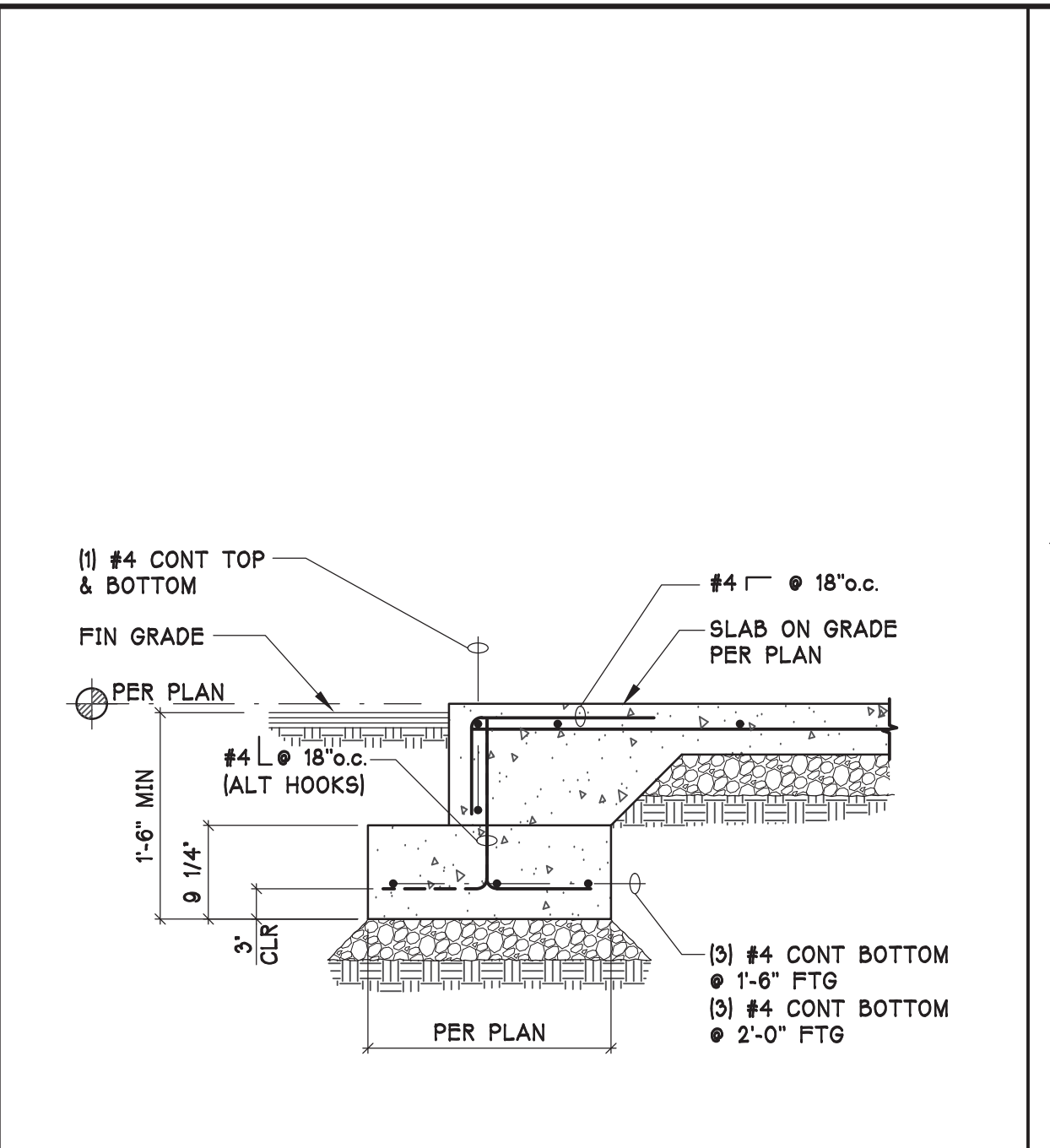
C SECTION 3/4" = 1'-0"
