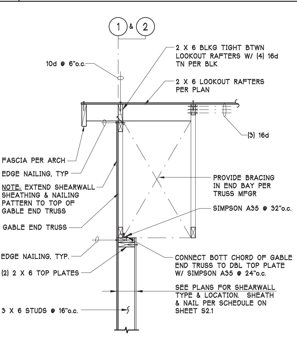
F SECTION 3/4" = 1'-0"
