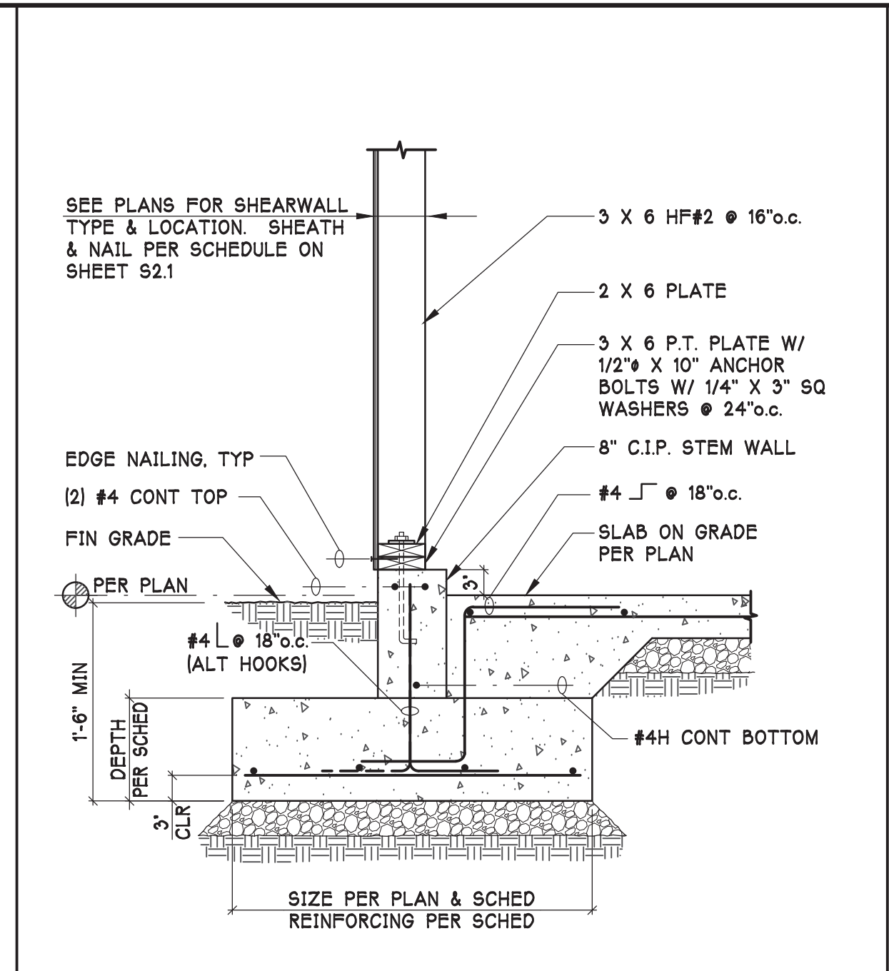
B SECTION 3/4" = 1'-0"
