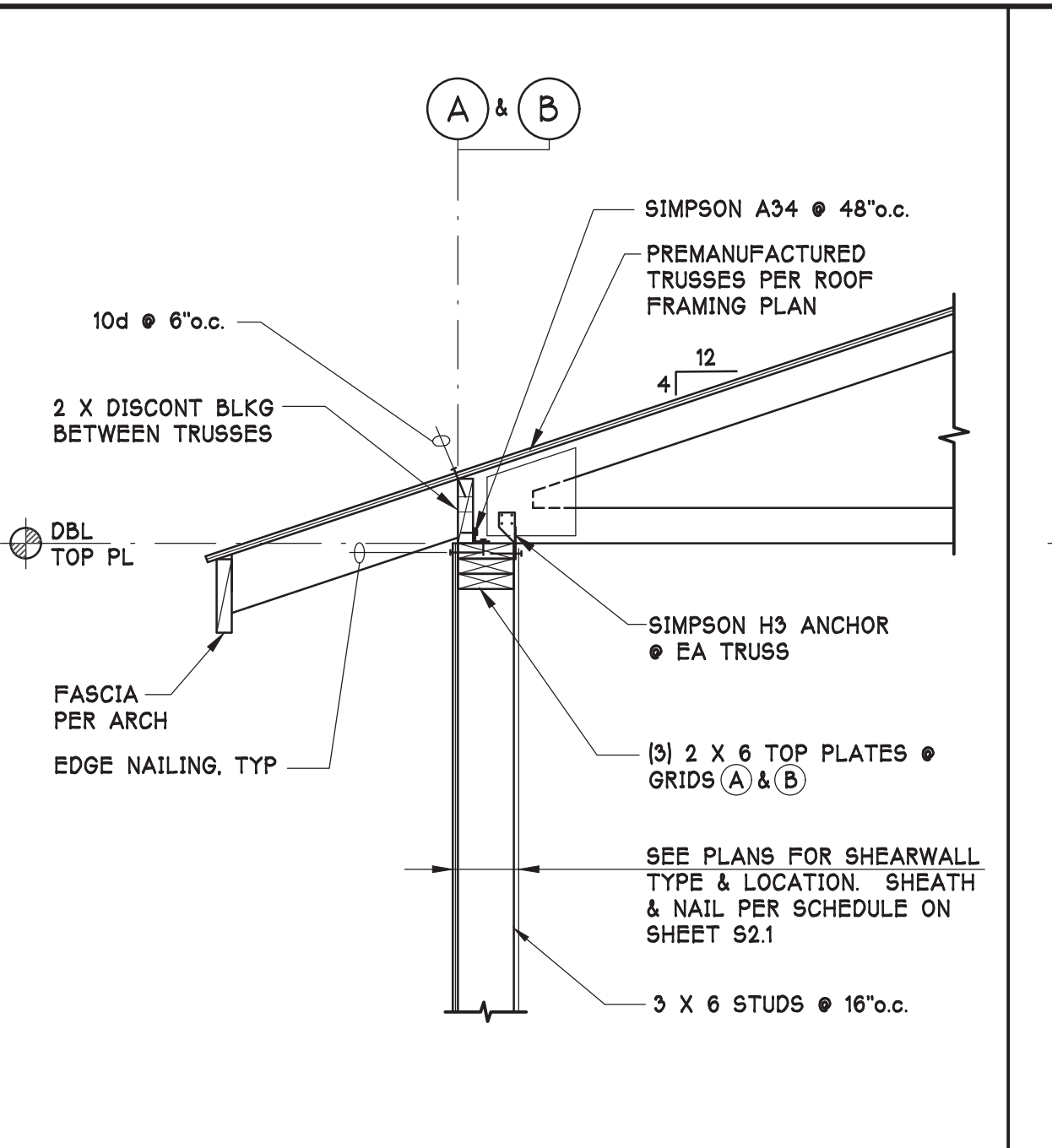
D SECTION 3/4" = 1'-0"
