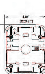
Wall Surface Mount Back Box SBBRL/SBBWL
