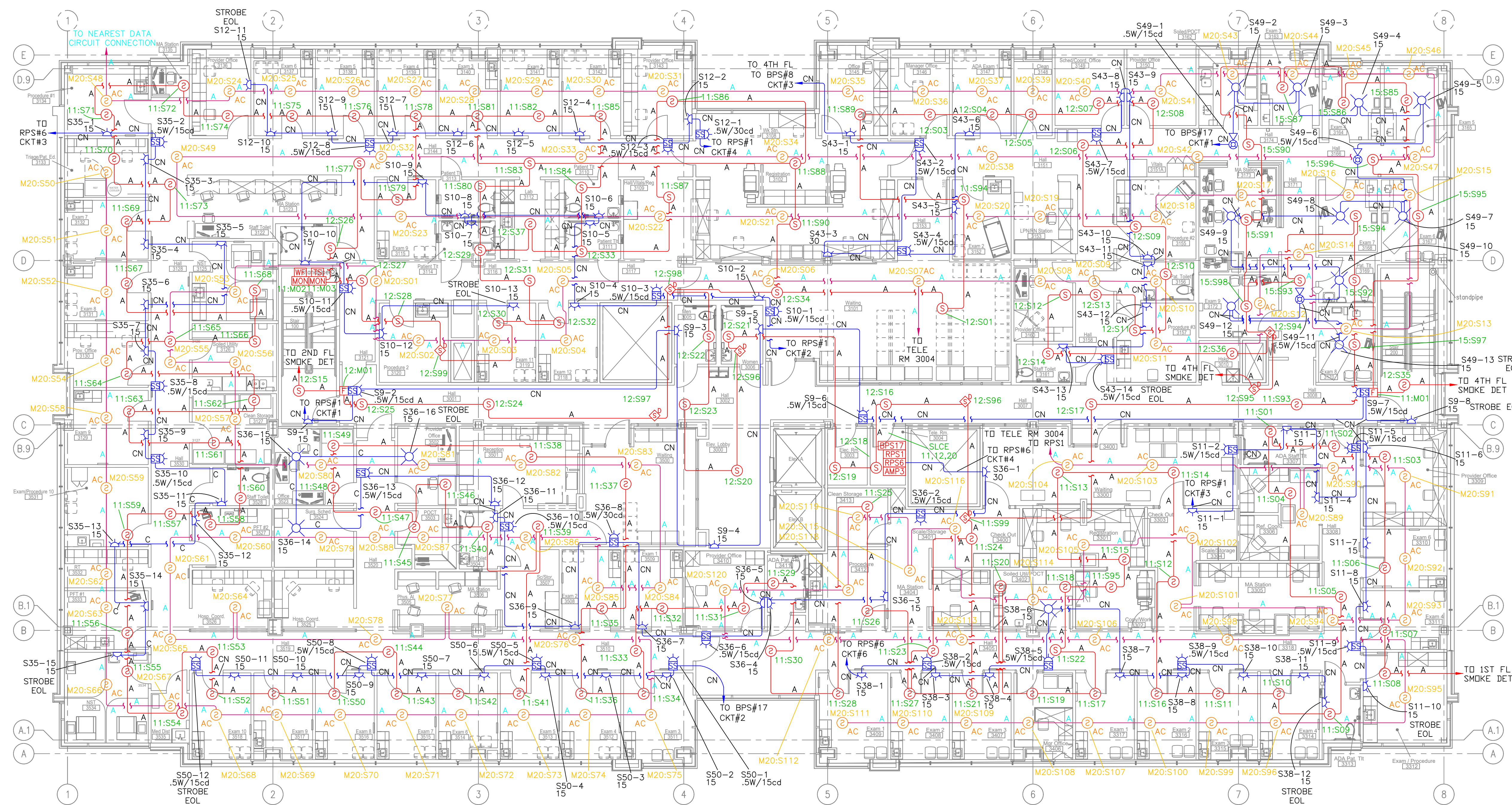
THIRD FLOOR - FIRE ALARM FLOOR PLAN SCALE: 1/8"=1'-0"
