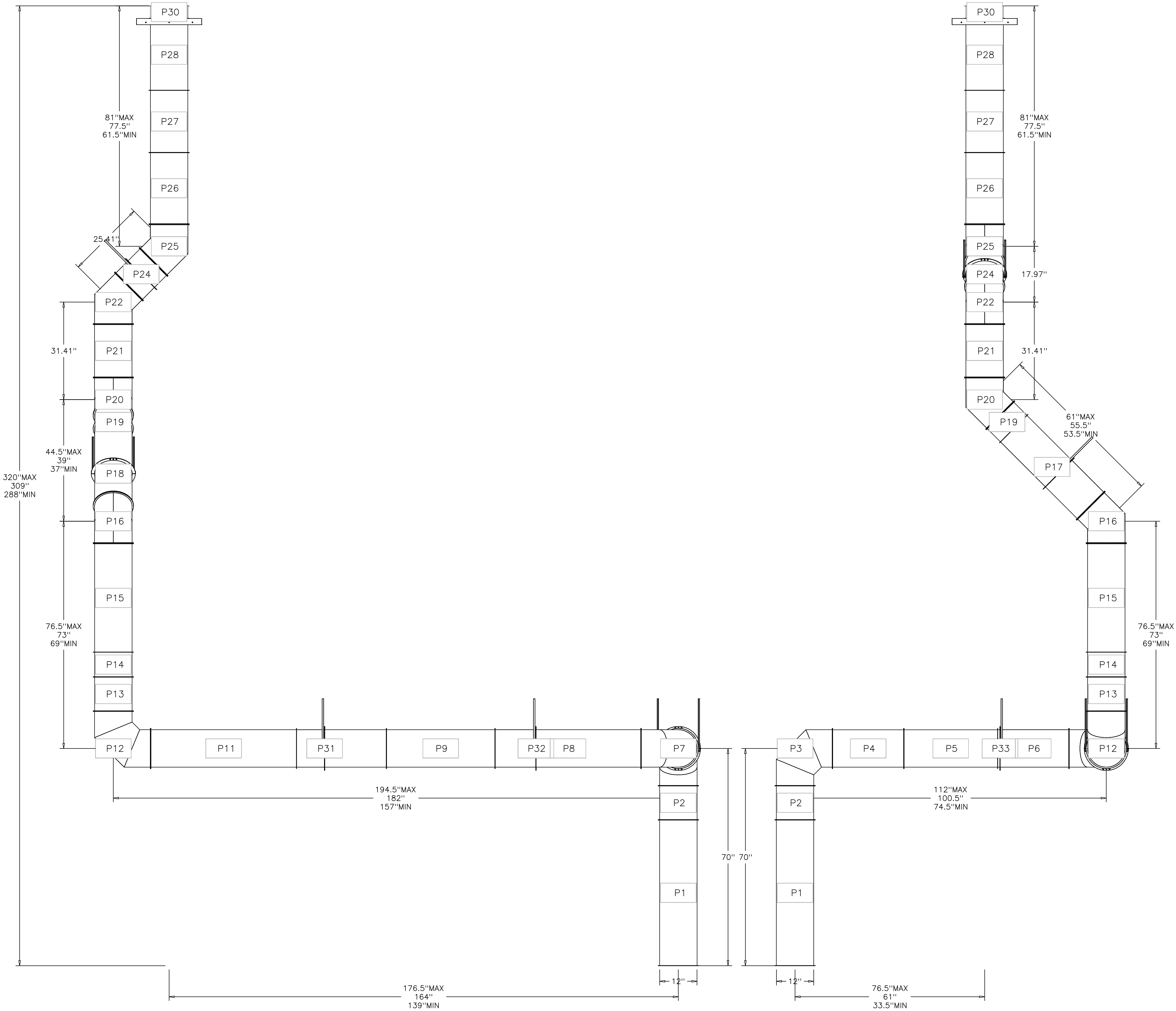
DUCTWORK #3 FRONT VIEW H-08
