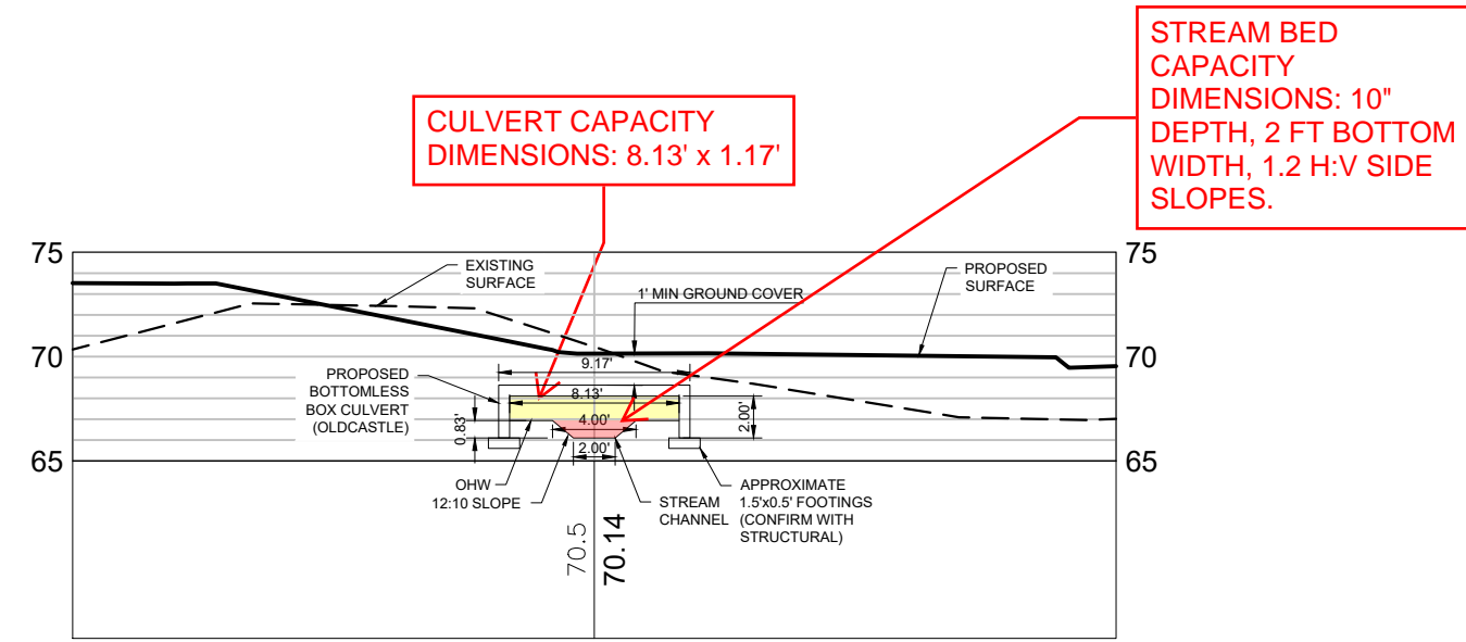
1 HPA APPROVED CULVERT 1 CROSS-SECTION SCALE 1"=10'
