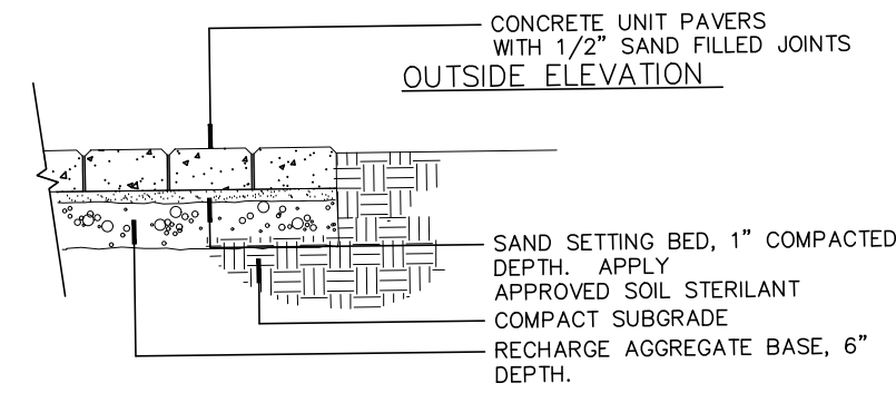
(J) PERVIOUS CONCRETE PAVERS
