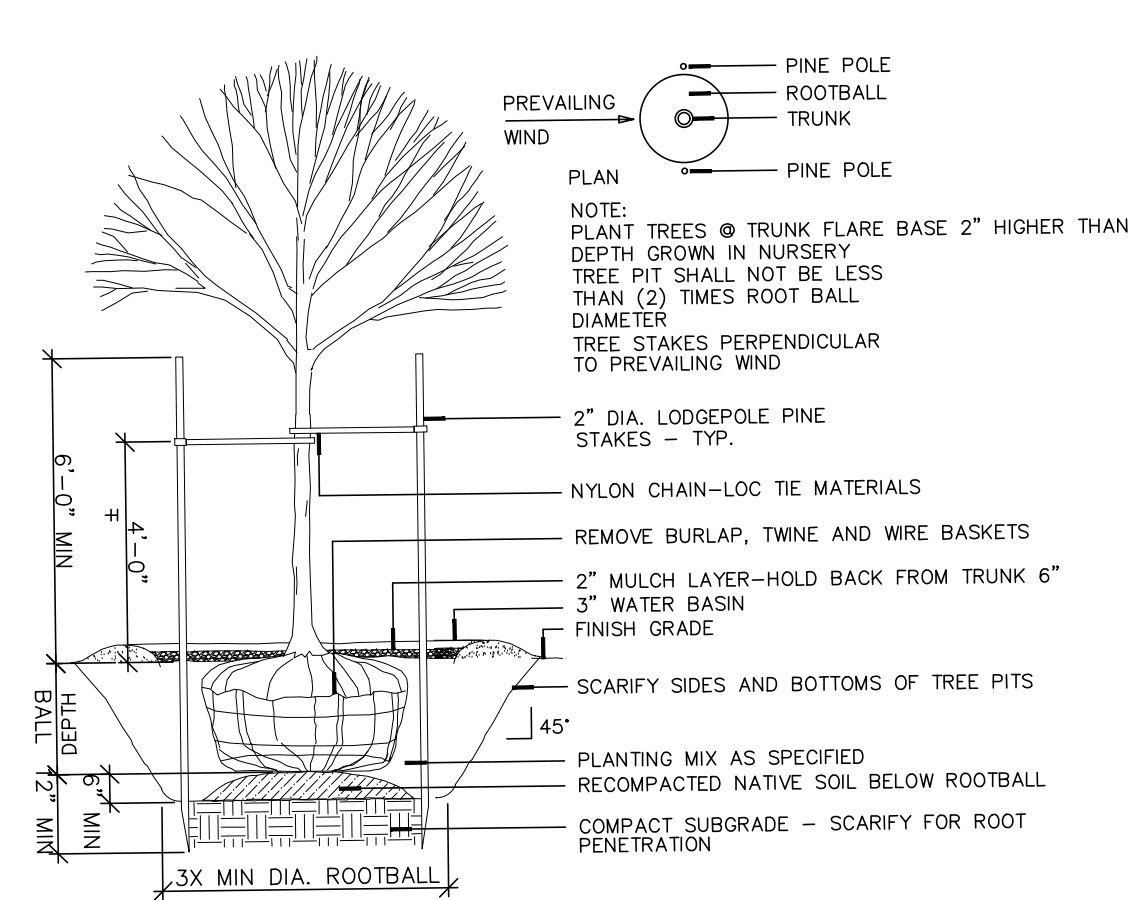
(A) TYPICAL DECIDUOUS TREE PLANTING NOT TO SCALE TREE-DECID
