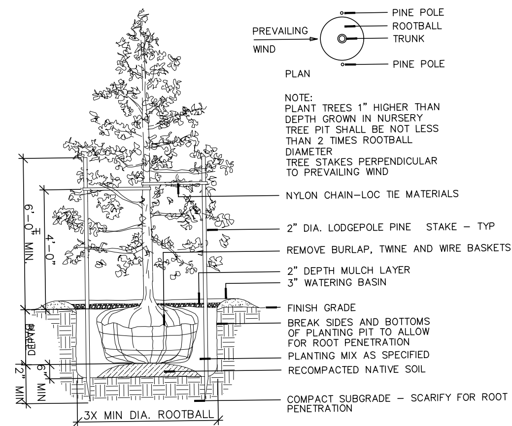
(B) TYPICAL CONIFEROUS TREE PLANTING NOT TO SCALE TREE-CONIF
