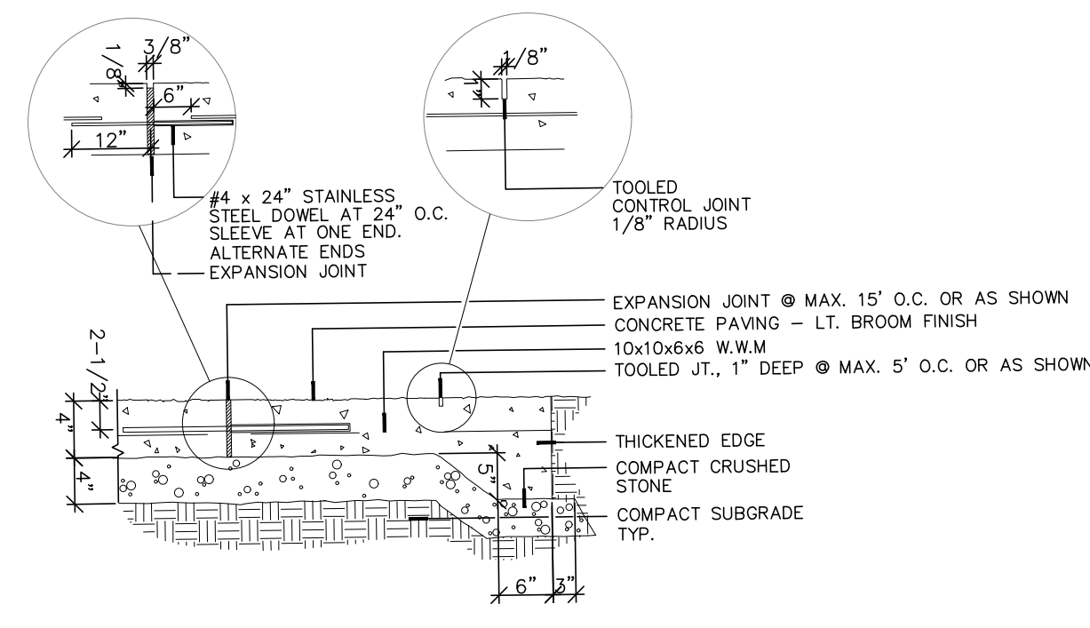
(K) TYPICAL CONCRETE PAVING NOT TO SCALE PAV-CONCS
