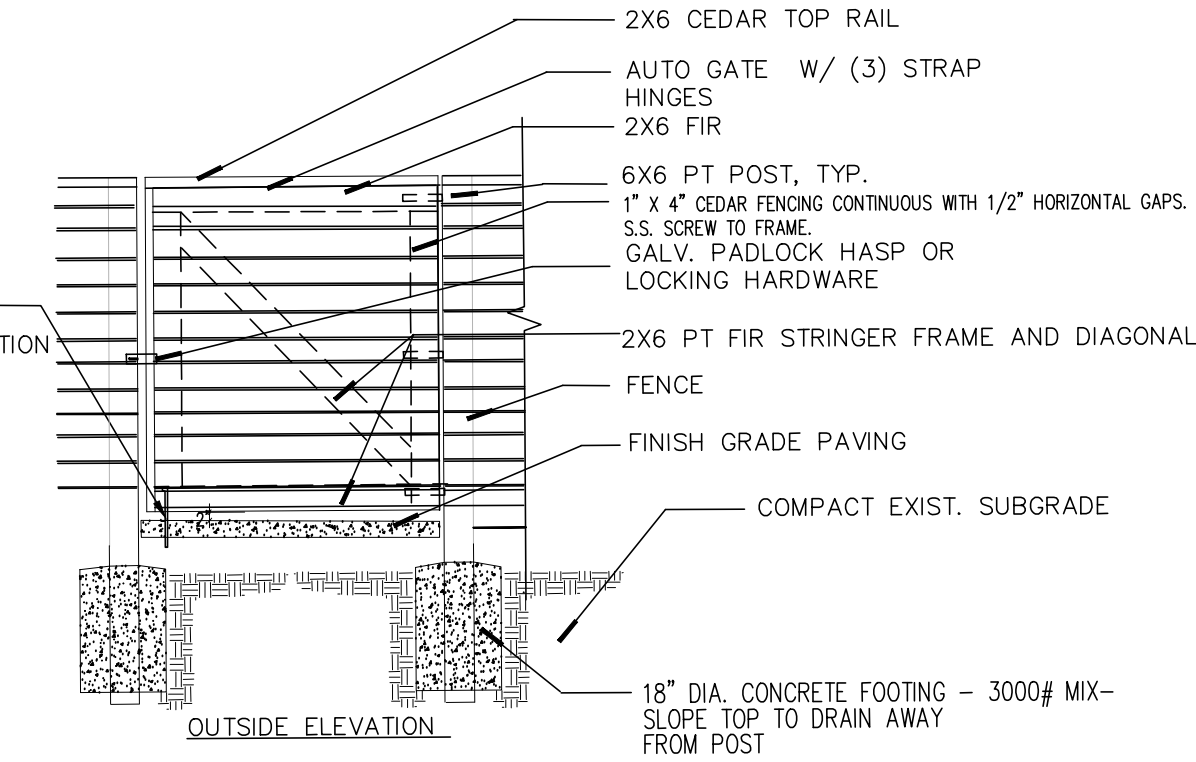
SWING WOOD GATE NOT TO SCALE
