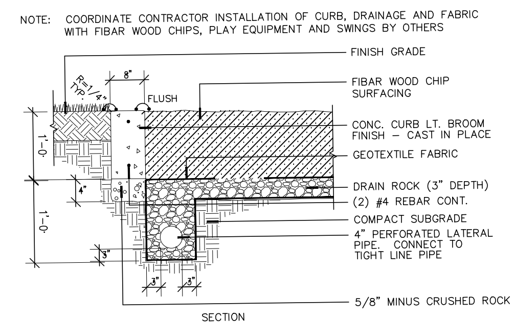
(H) CONCRETE CURB @ PLAY AREA W/ SOFT SURFACING N.T.S. PLAYSURF-2
