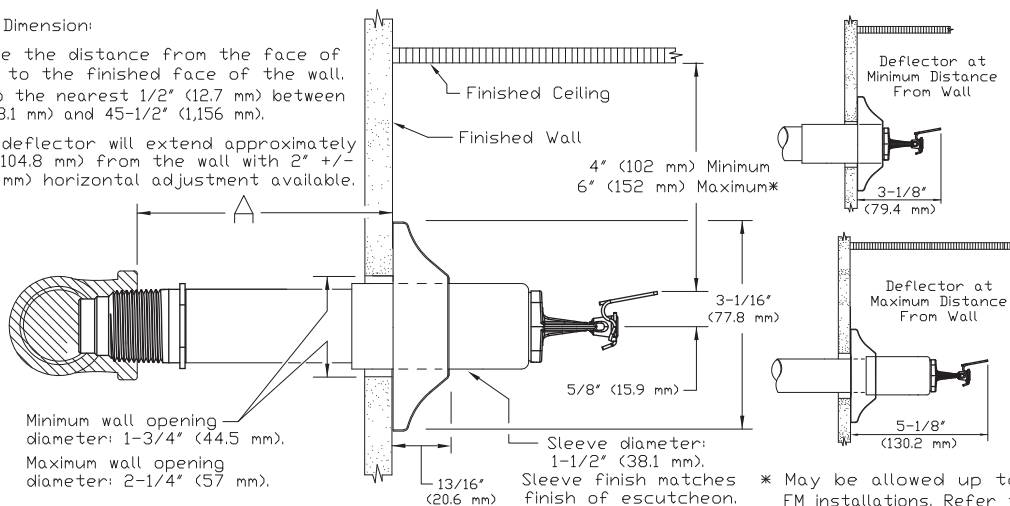
Figure 3: Adjustable Standard Dry Horizontal Sidewall Sprinkler
