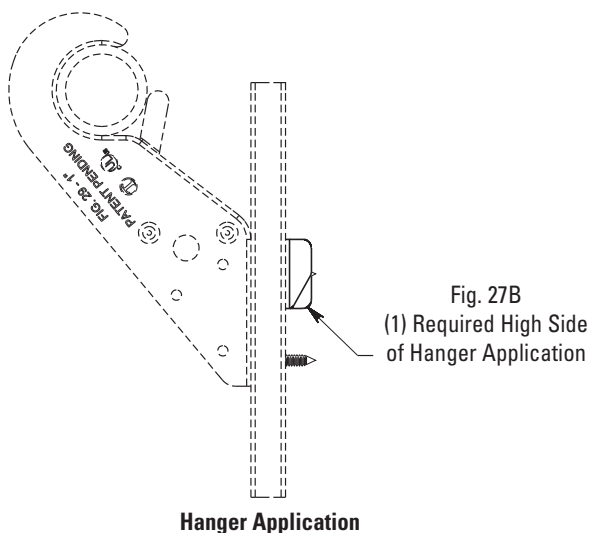
Hanger Application
