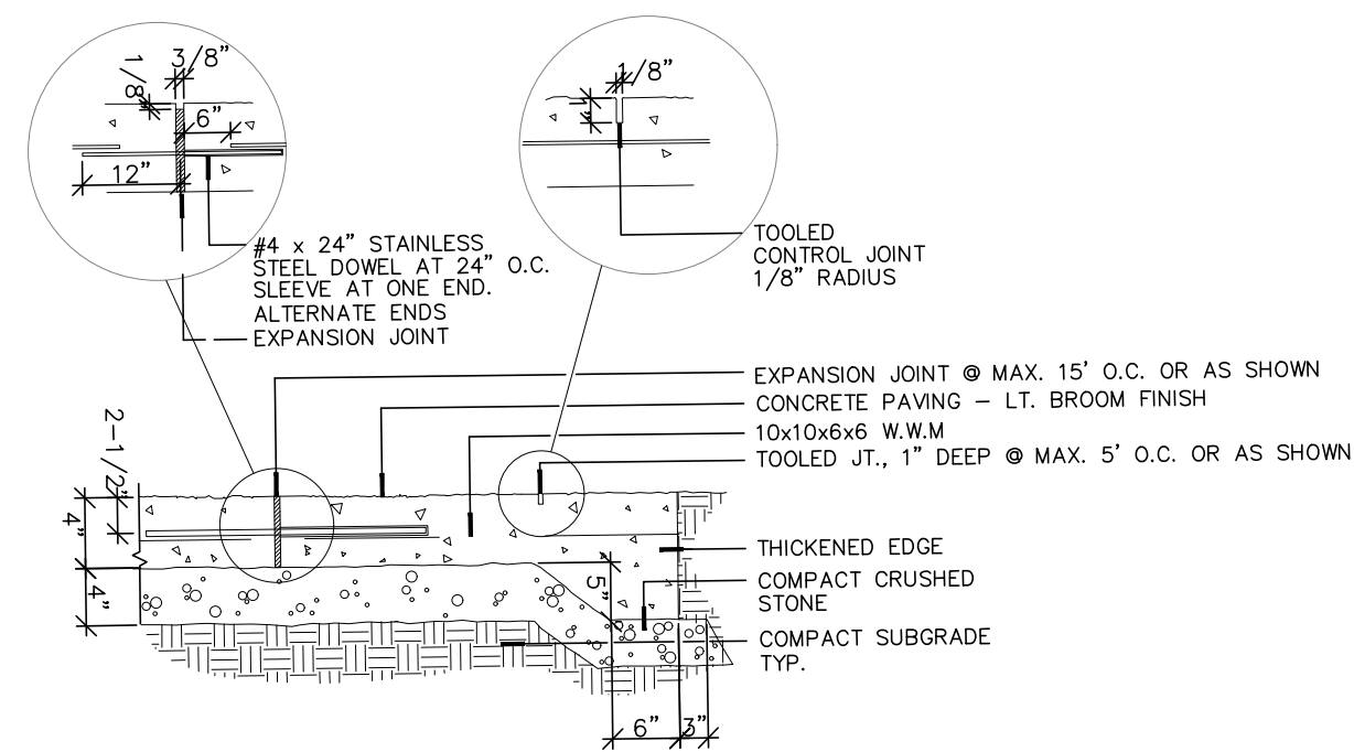
K TYPICAL CONCRETE PAVING NOT TO SCALE
