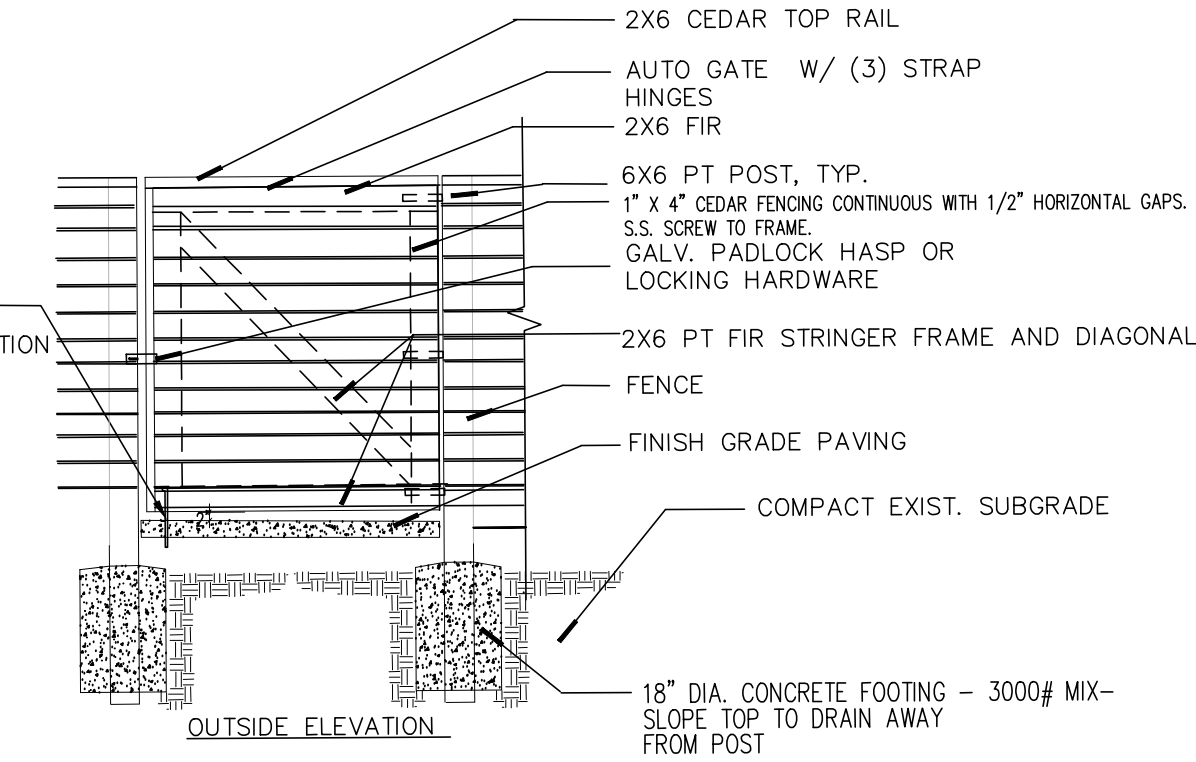
K SWING WOOD GATE NOT TO SCALE
