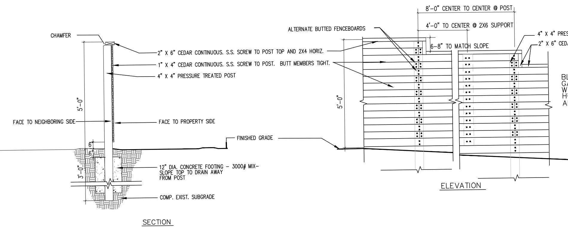
G SOLID SCREEN FENCE/SWING WOOD GATE NOT TO SCALE
