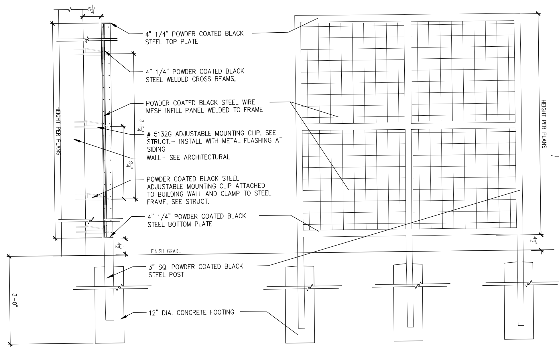
F GREEN SCREEN FOR VEGETATED WALL NOT TO SCALE
