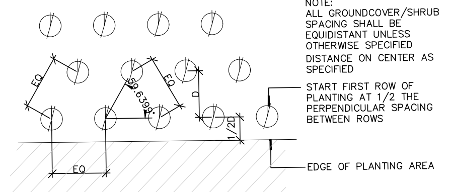
E TRIANGULAR PLANT SPACING NOT TO SCALE
