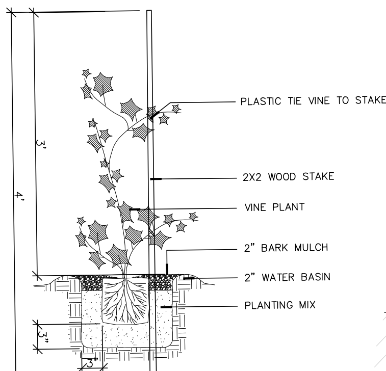
D STAKED VINE PLANTING NOT TO SCALE
