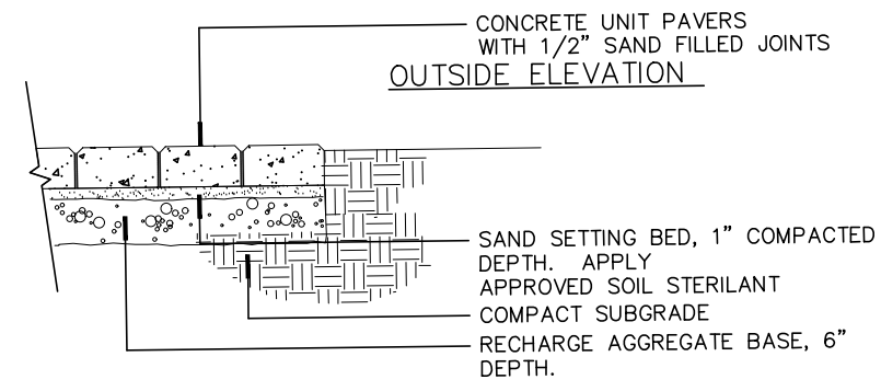
J PERVIOUS CONCRETE PAVERS
