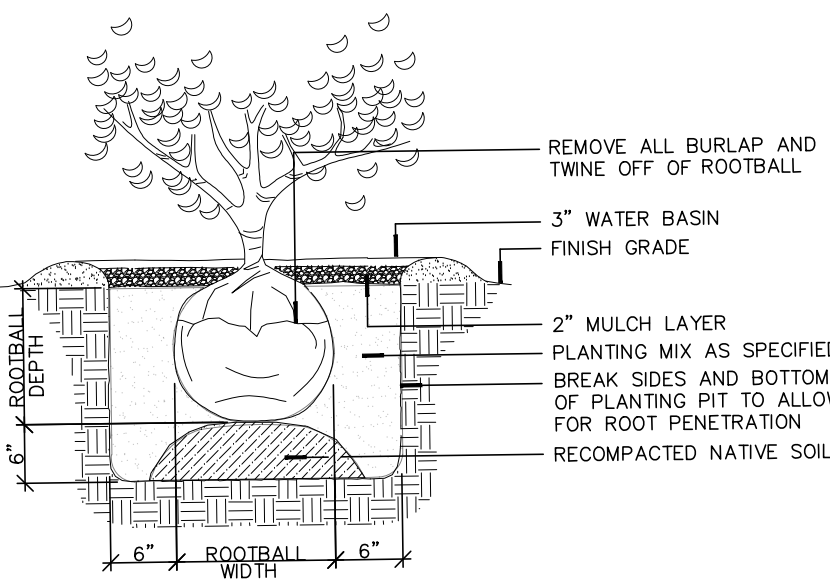
C TYPICAL SHRUB PLANTING DETAIL NOT TO SCALE
