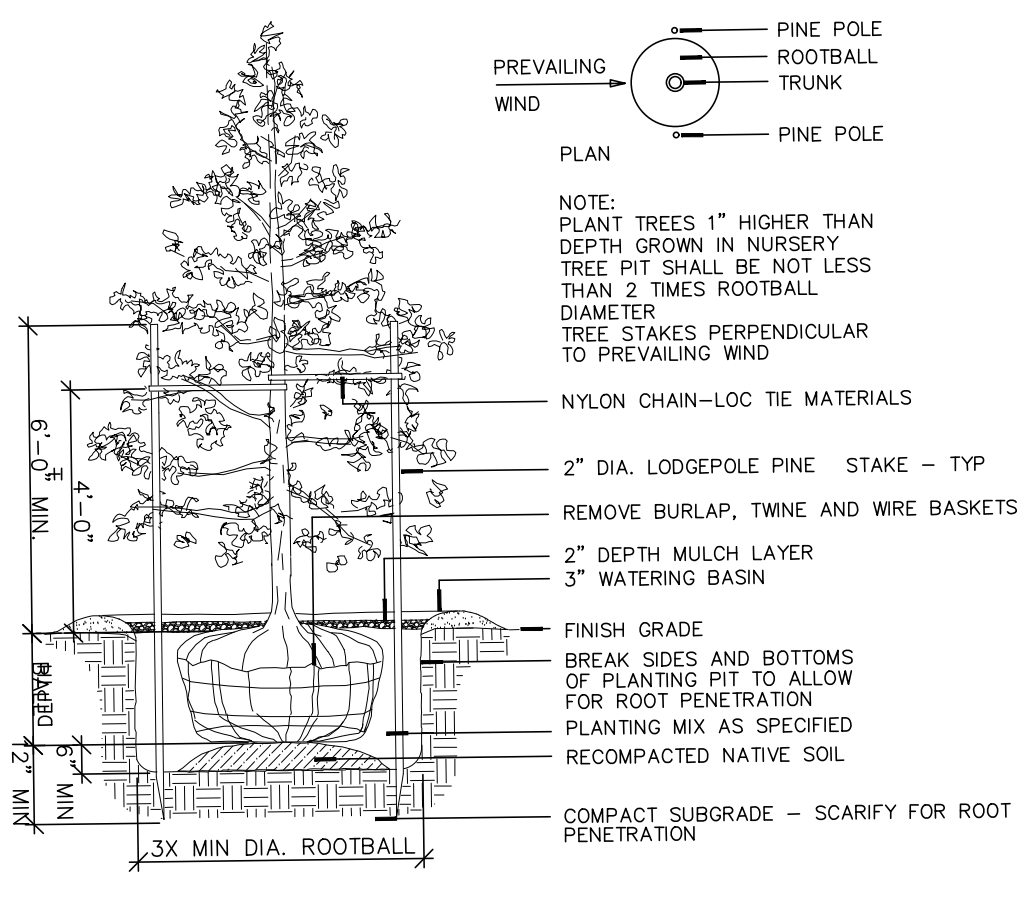
B TYPICAL CONIFEROUS TREE PLANTING NOT TO SCALE
