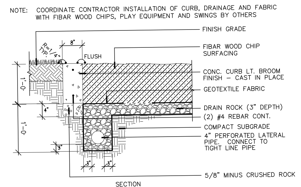
H CONCRETE CURB @ PLAY AREA W/ SOFT SURFACING N.T.S. PLAYSURF-2
