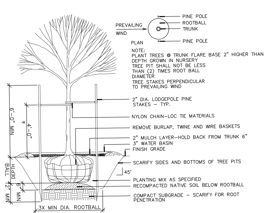
A TYPICAL DECIDUOUS TREE PLANTING NOT TO SCALE
