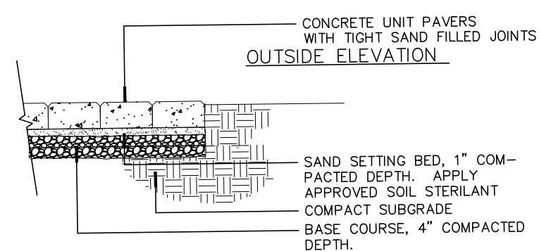
I IMPERVIOUS CONCRETE PAVERS
