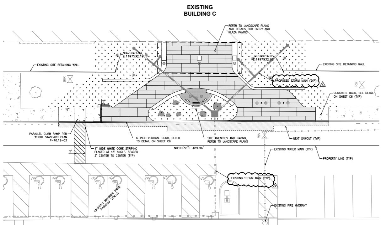
PPSB FRONT ENTRANCE SCALE: 1" = 10'
