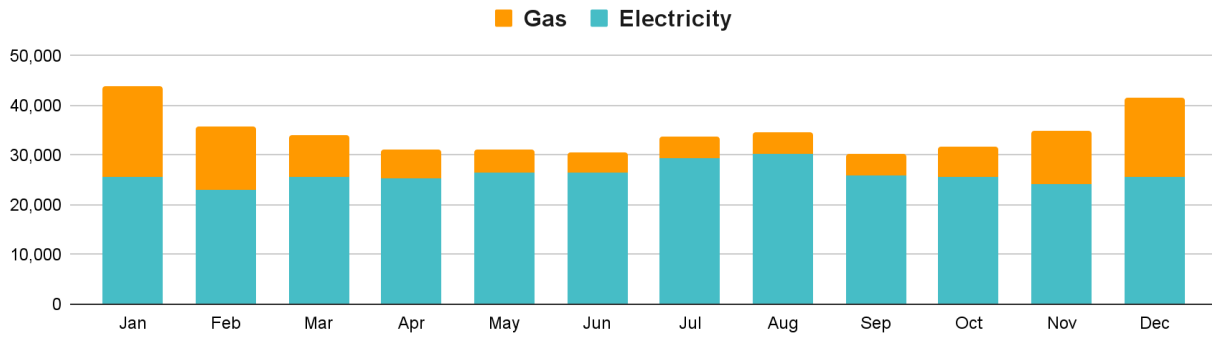
Baseline Energy Consumption [kBtu]
