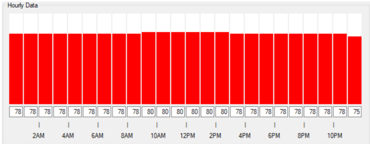
Graph-5.5.7: Retail Cooling Schedule (Temperature F)
