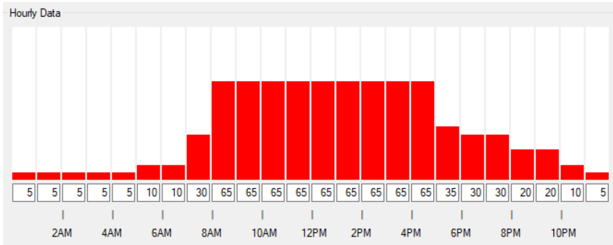
Graph-5.5.2: Retail Process Lighting Schedule (%)
