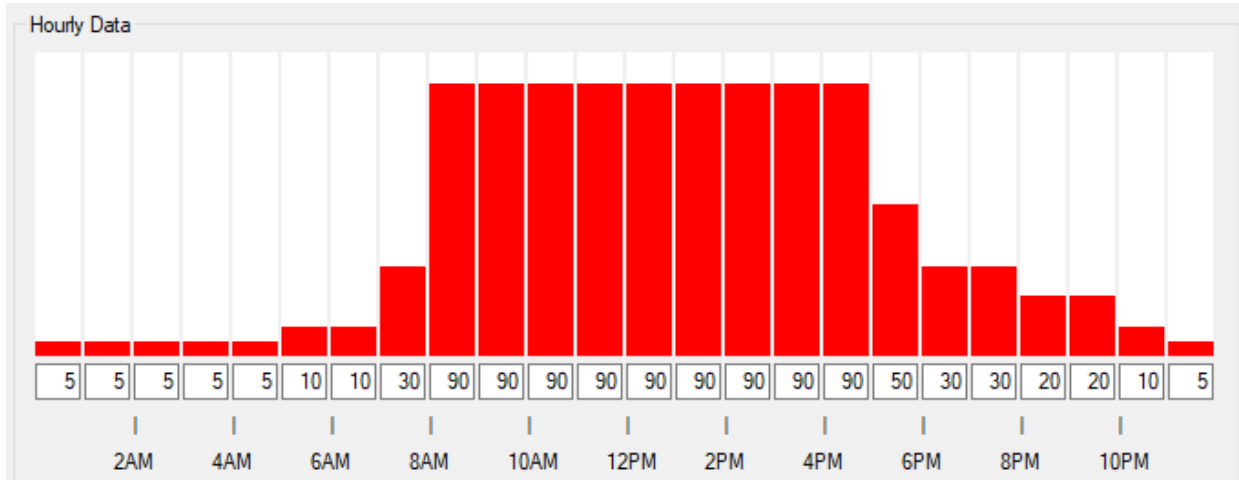
Graph-5.5.5: Retail Process Load Schedule (%)
