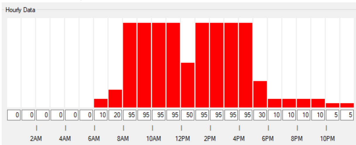
Graph-5.5.3: Retail tifamily Occupants Schedule (%)
