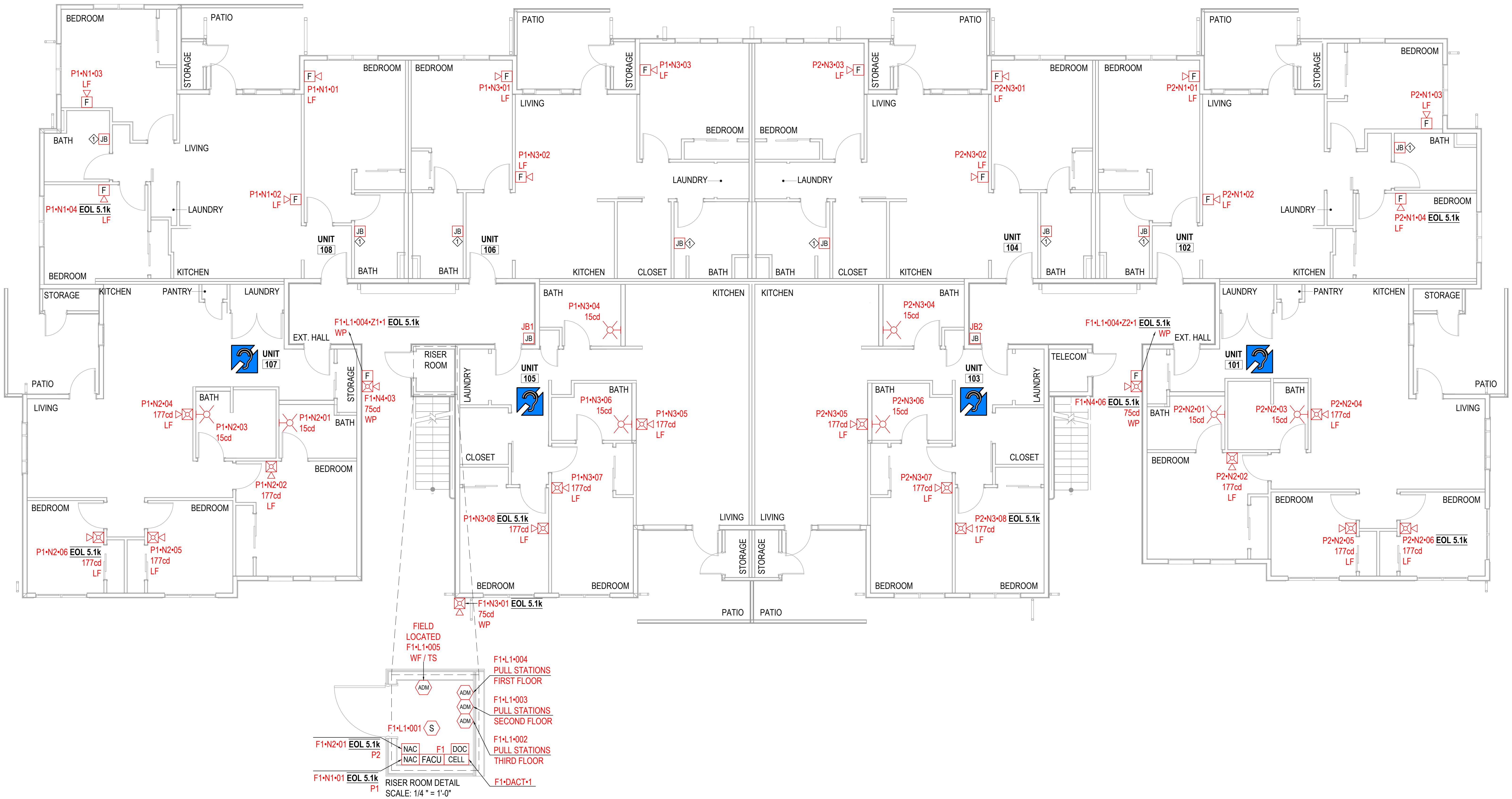
1 FIRST FLOOR PLAN 0 1' 5' 10' 3/16" = 1'-0"
