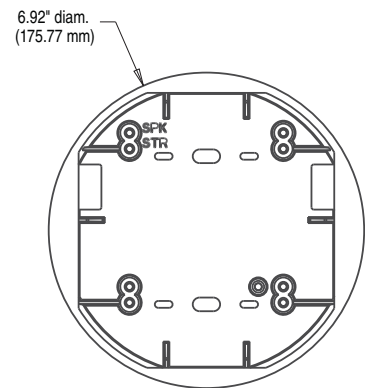
Surface Mount Back Box for Ceilings (SBBCL, SBCWL)
