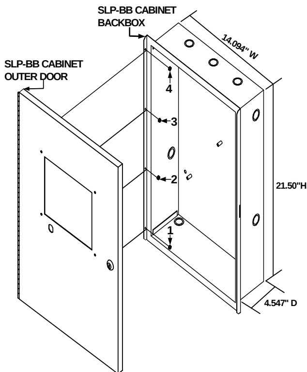
Figure 2 SLP Enclosure
