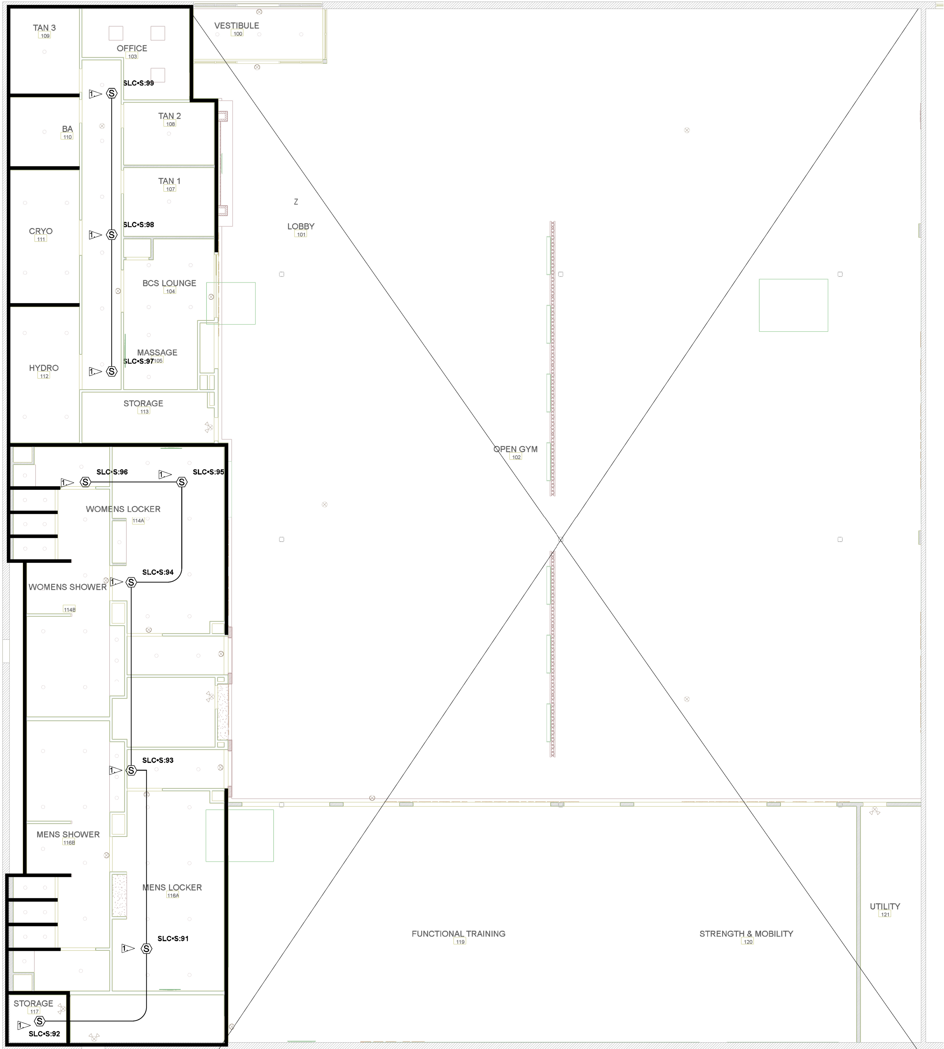
INITIATION PLAN (ABOVE CEILING) SCALE: 1/8"=1'-0"
