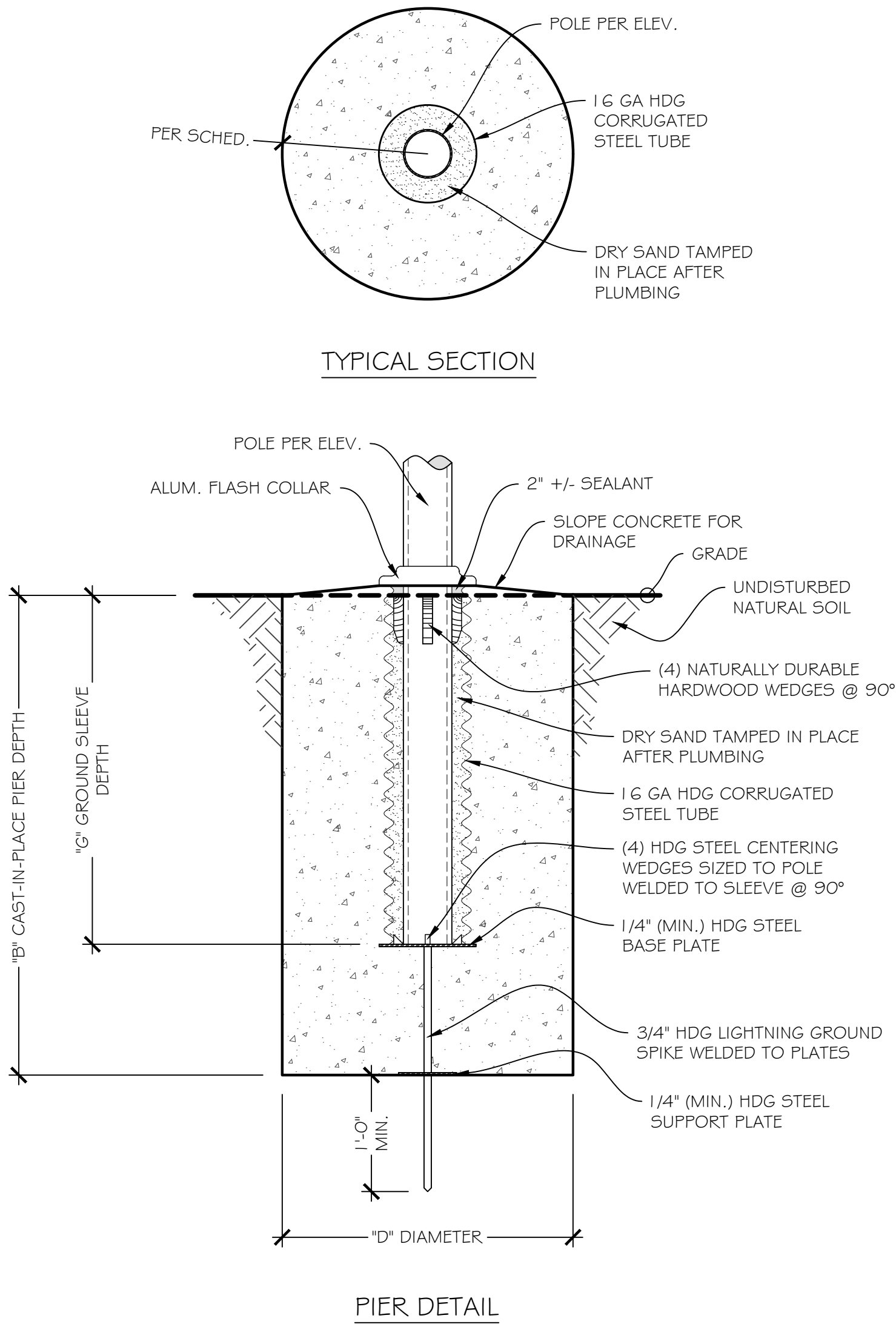
2 FOUNDATION DETAIL
