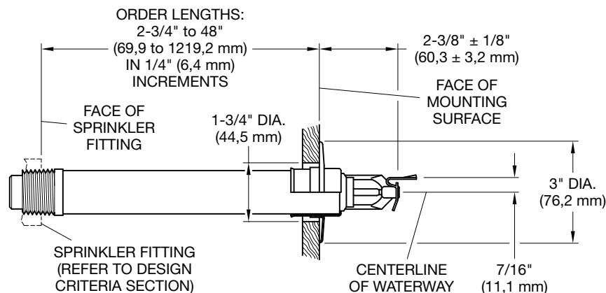
FIGURE 2 EXTENDED COVERAGE HORIZONTAL SIDEWALL WITH STANDARD ESCUTCHEON TY3338 (3 MM BULB) AND TY3358 (5 MM BULB)
