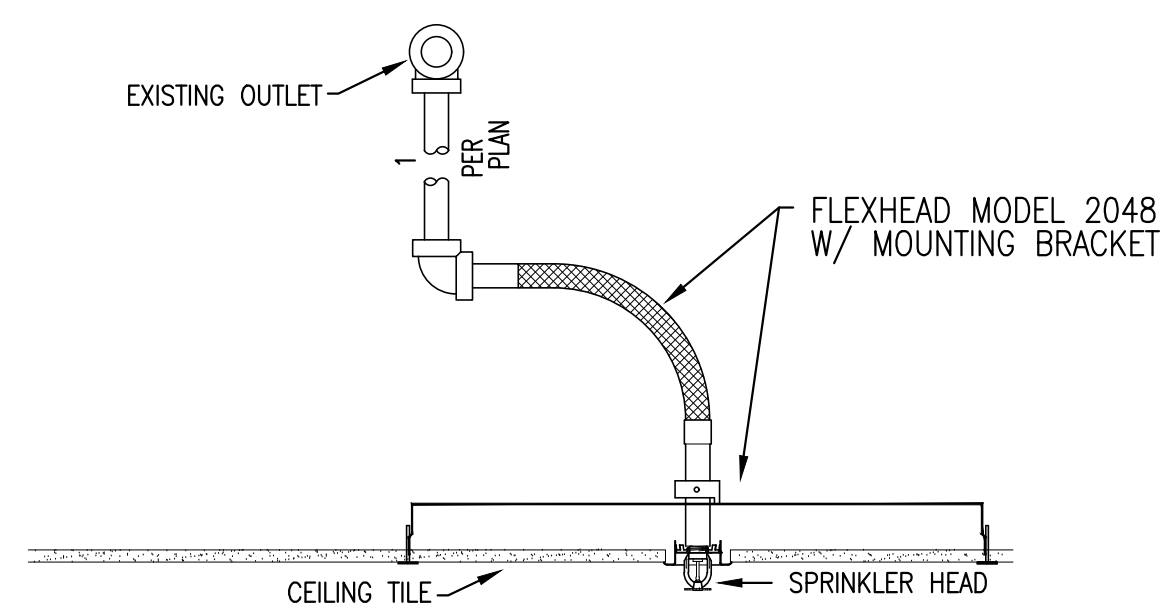
FLEXIBLE SPRINKLER DETAIL
