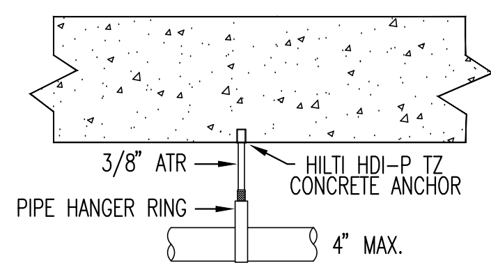
TYPICAL HANGER DETAIL
