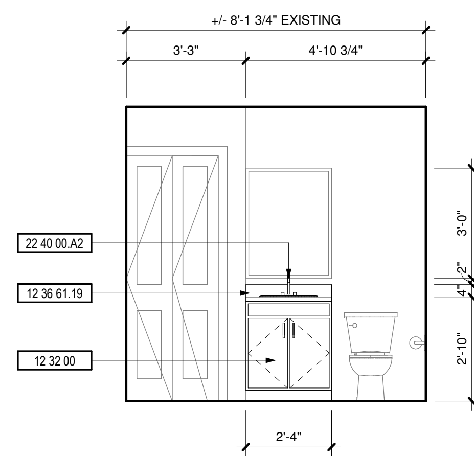
12 BATHROOM 3/8" = 1'-0"
