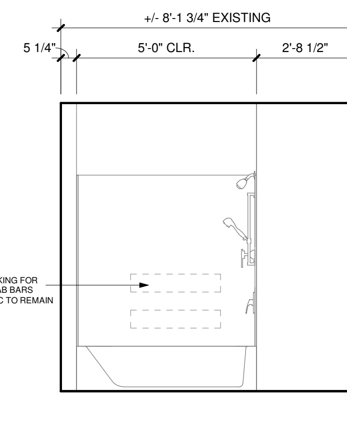
7 BATHROOM (ADA) 3/8" = 1'-0"
