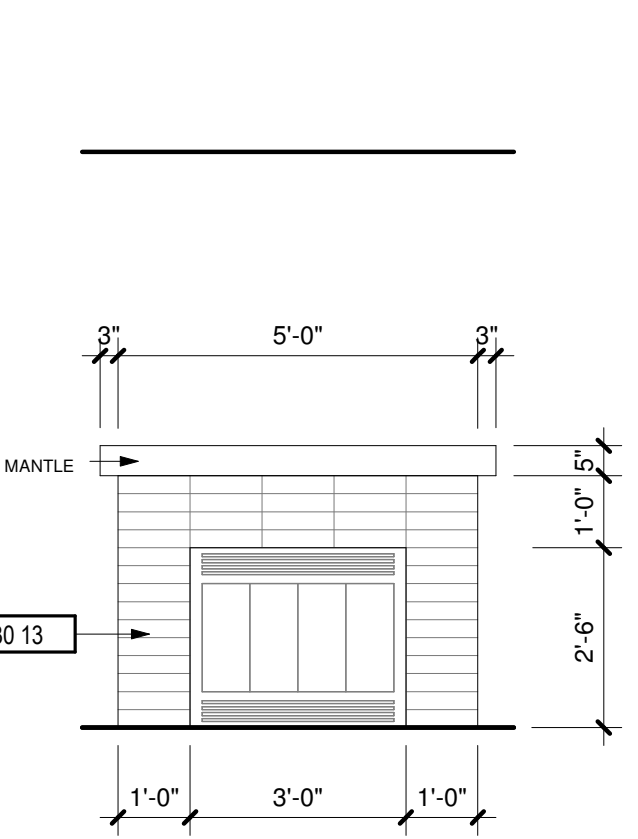
7 FIREPLACE 3/8" = 1'-0"
