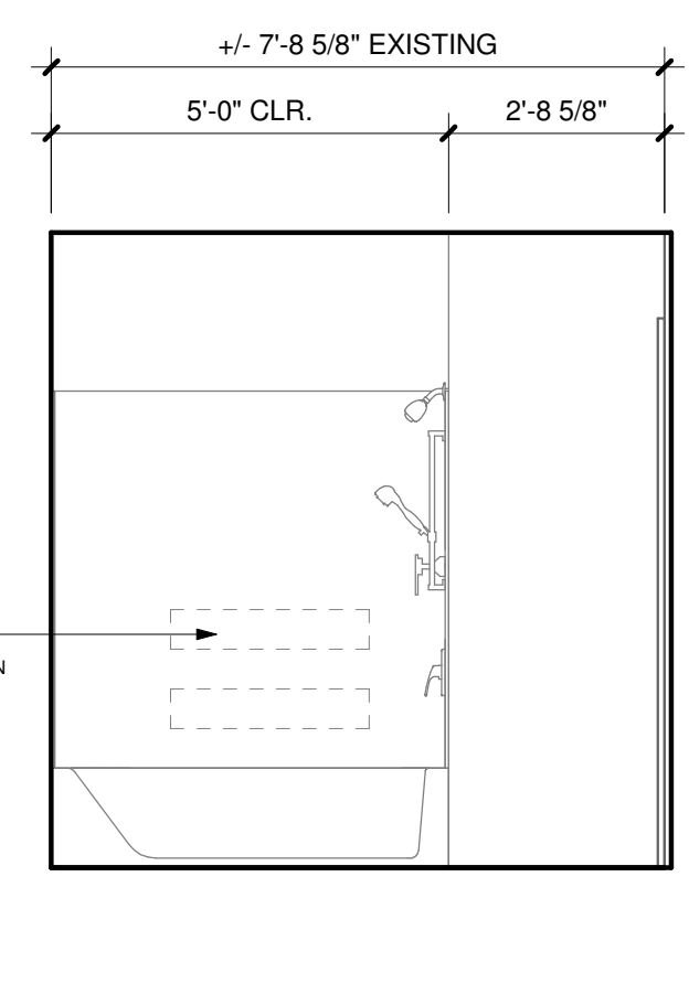
5 BATHROOM (ADA) 3/8" = 1'-0"
