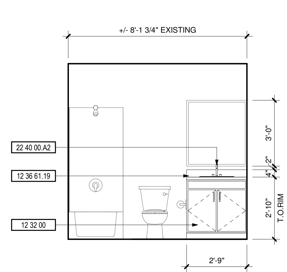
8 BATHROOM 3/8" = 1'-0"
