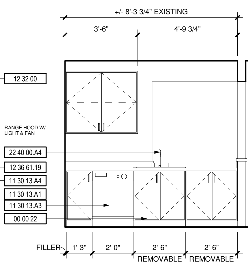
2 KITCHEN (ADA) 3/8" = 1'-0"
