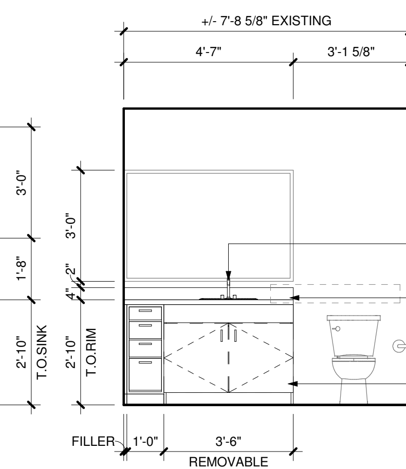
3 BATHROOM (ADA) 3/8" = 1'-0"
