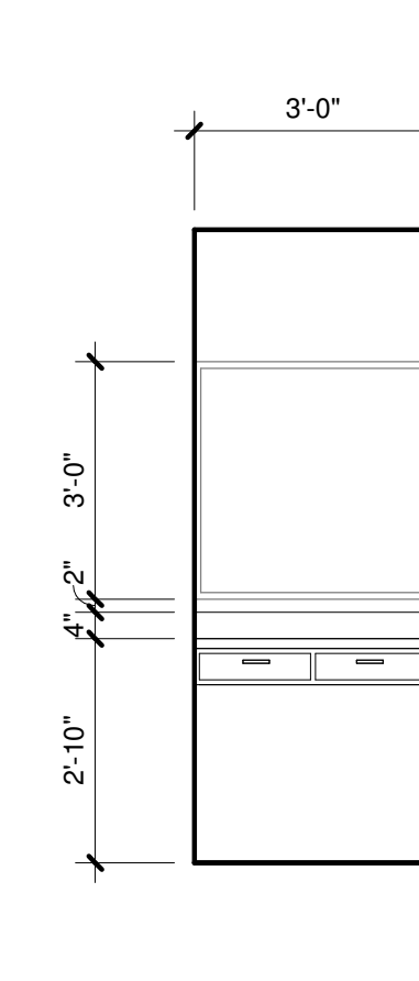
13 VANITY 3/8" = 1'-0"
