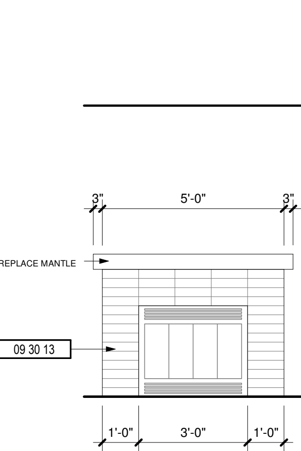
9 FIREPLACE 3/8" = 1'-0"
