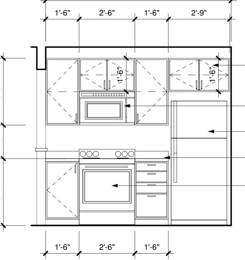
8 KITCHEN 3/8" = 1'-0"
