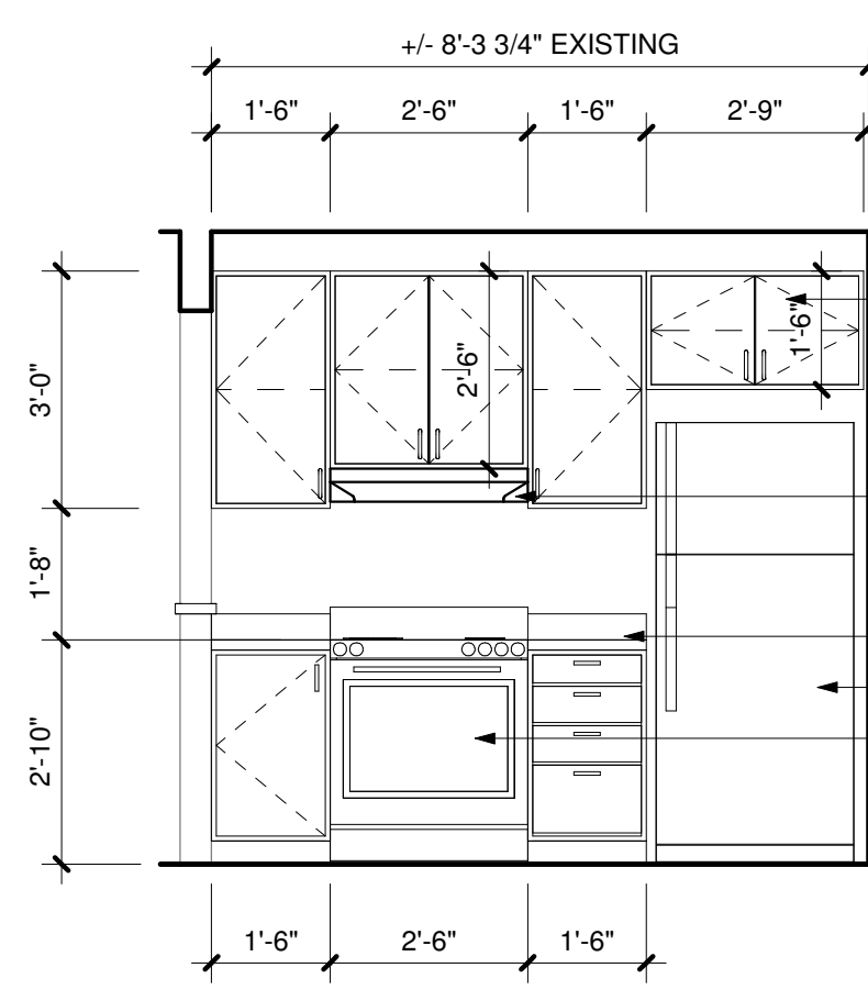
1 KITCHEN (ADA) 3/8" = 1'-0"
