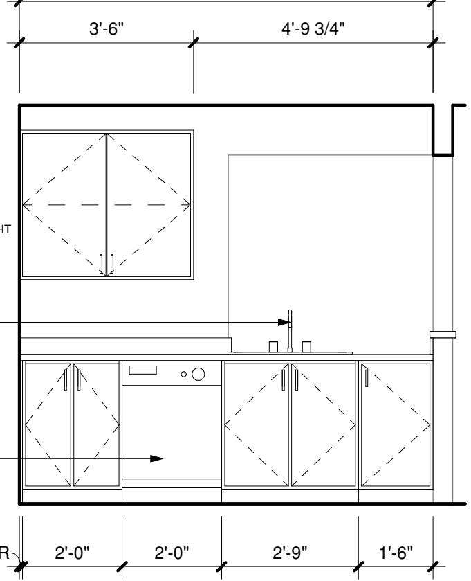
9 KITCHEN 3/8" = 1'-0"
