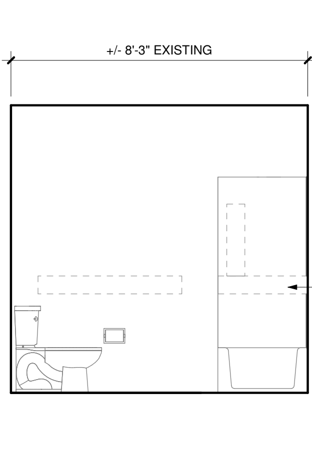
4 BATHROOM (ADA) 3/8" = 1'-0"
