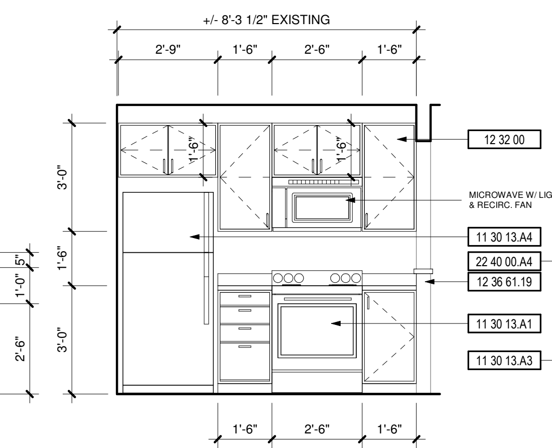
10 KITCHEN 3/8" = 1'-0"
