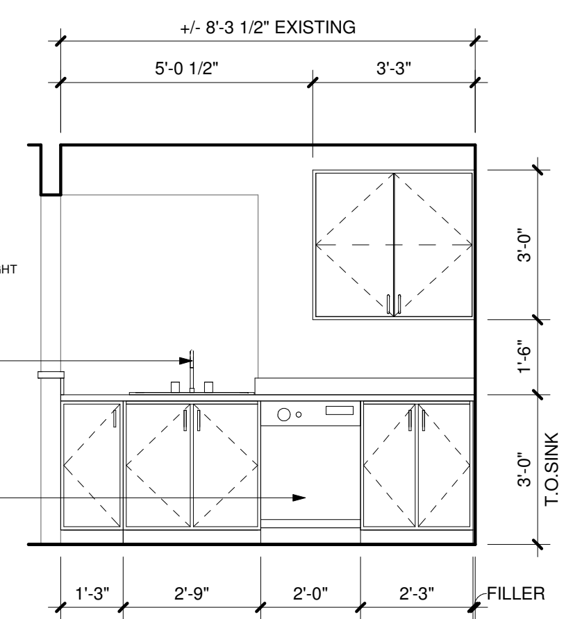
11 KITCHEN 3/8" = 1'-0"
