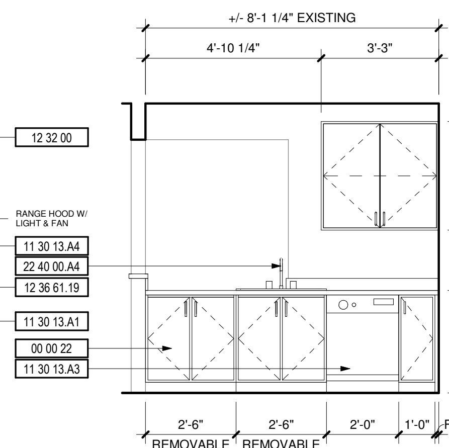
4 KITCHEN (ADA) 3/8" = 1'-0"
