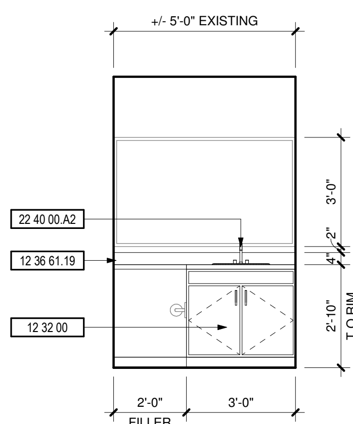
6 BATHROOM 3/8" = 1'-0"
