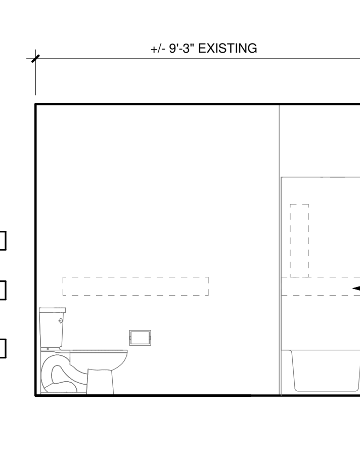
6 BATHROOM (ADA) 3/8" = 1'-0"
