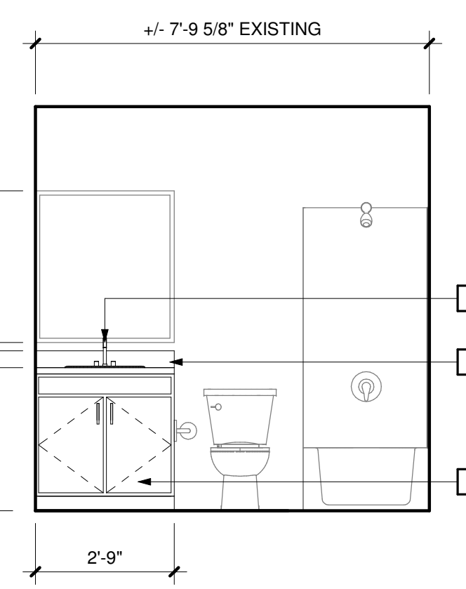
10 BATHROOM 3/8" = 1'-0"
