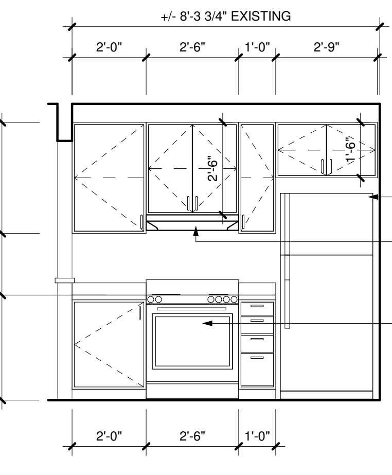
4 KITCHEN (ADA) 3/8" = 1'-0"
