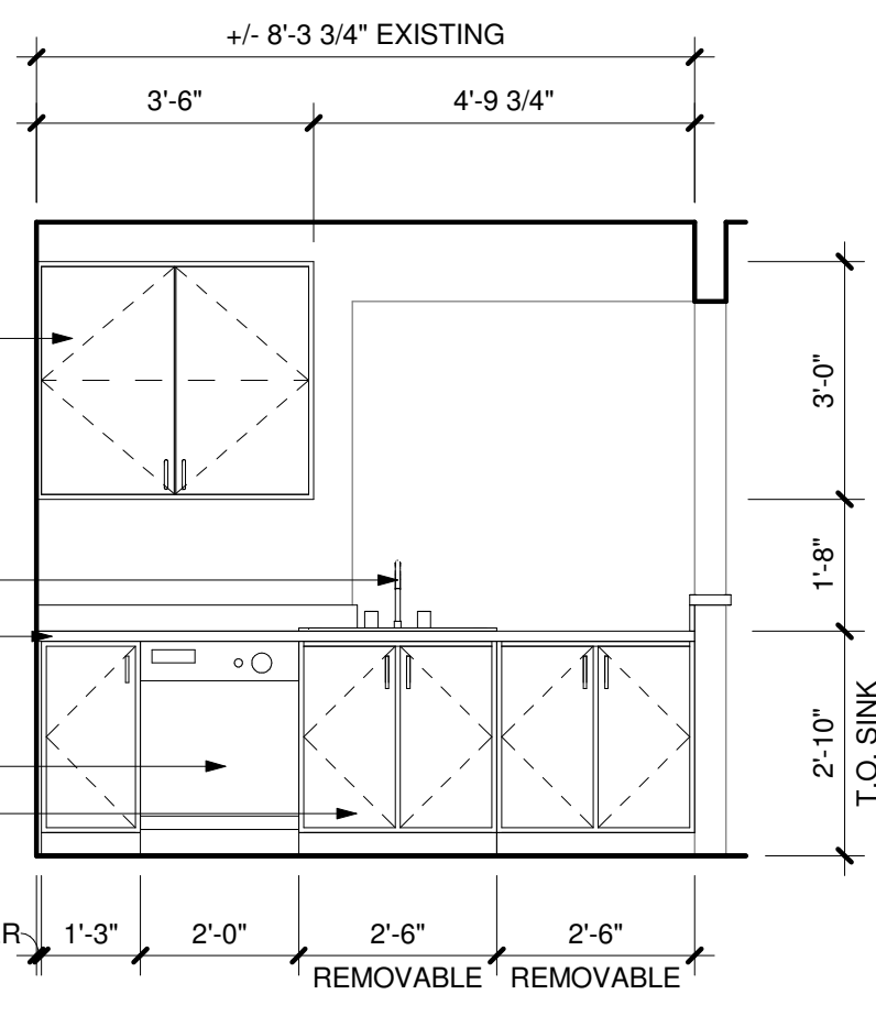
5 KITCHEN (ADA) 3/8" = 1'-0"
