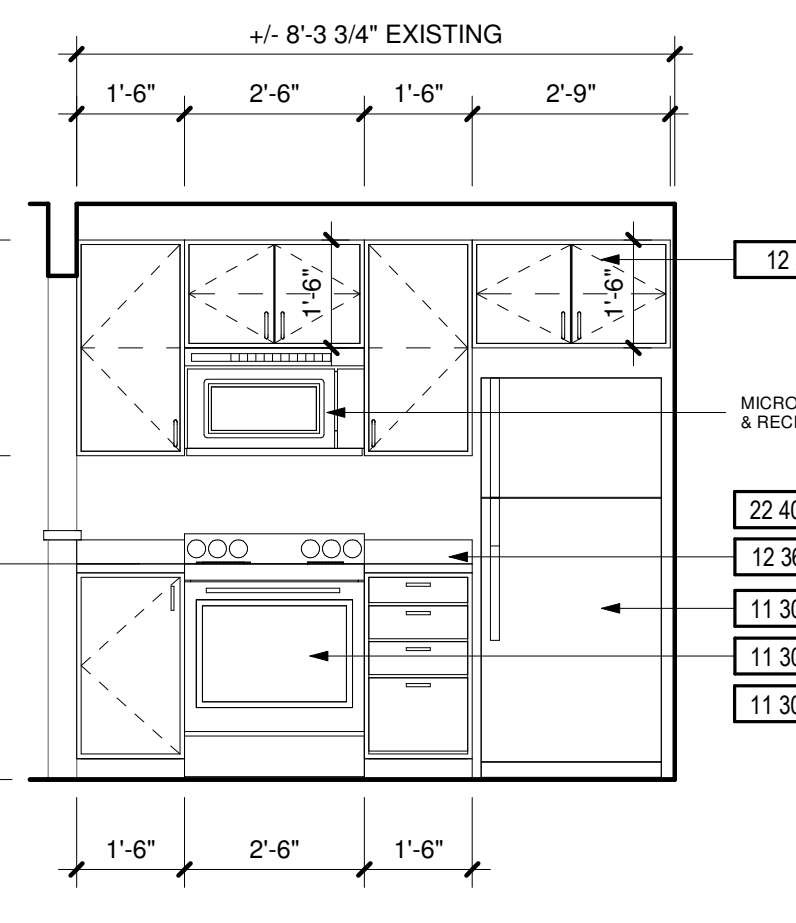
10 KITCHEN 3/8" = 1'-0"
