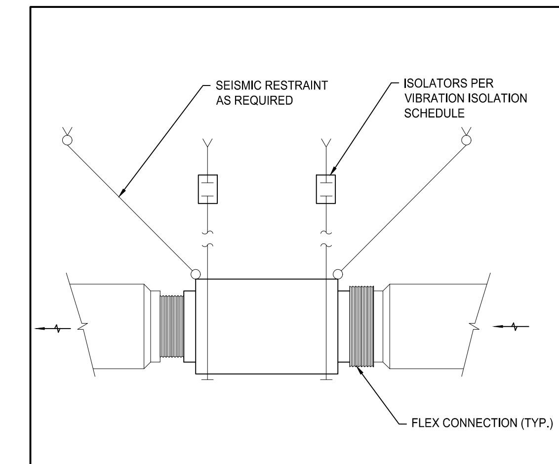
5 TM6.01 HORIZONTAL INLINE FAN DETAIL N.T.S.
