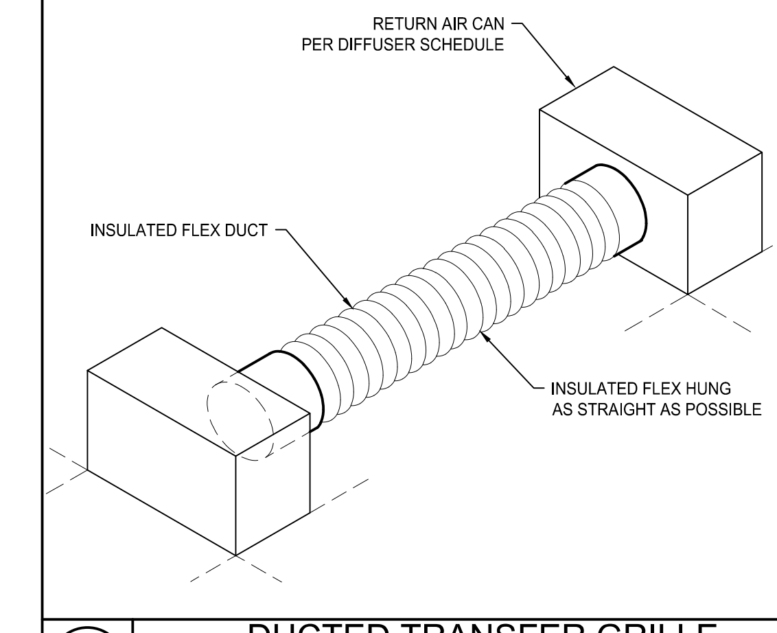
2 TM6.01 DUCTED TRANSFER GRILLE INSTALLATION DETAIL N.T.S.
