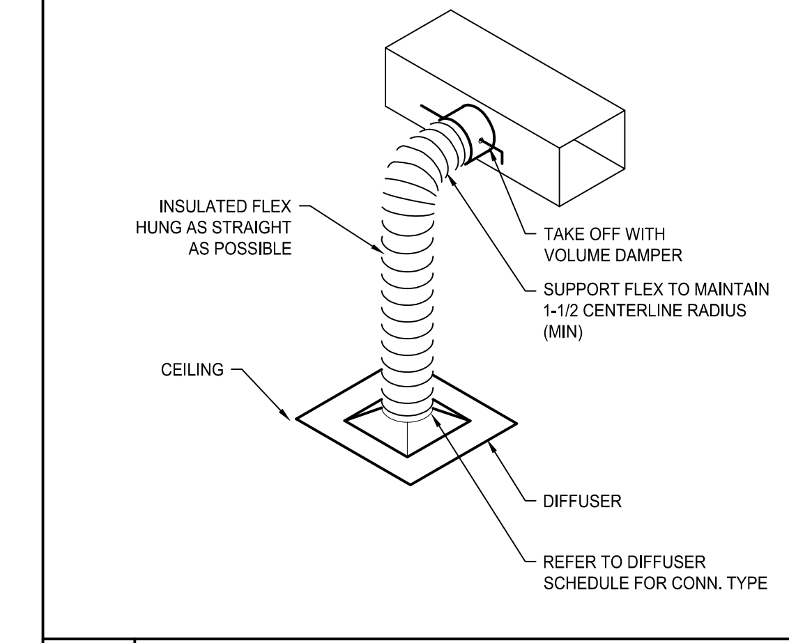
3 TM6.01 DIFFUSER INSTALLATION DETAIL N.T.S.
