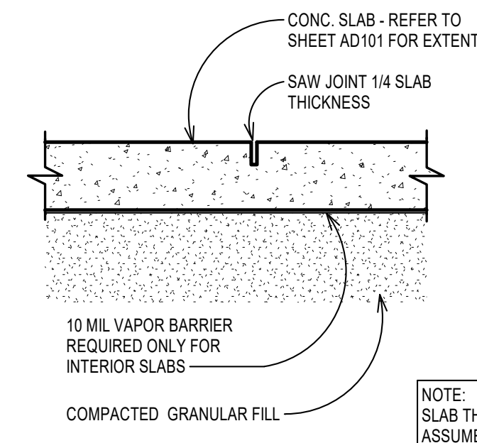
4 CONTROL JOINT SCALE: 1" = 1'-0"
