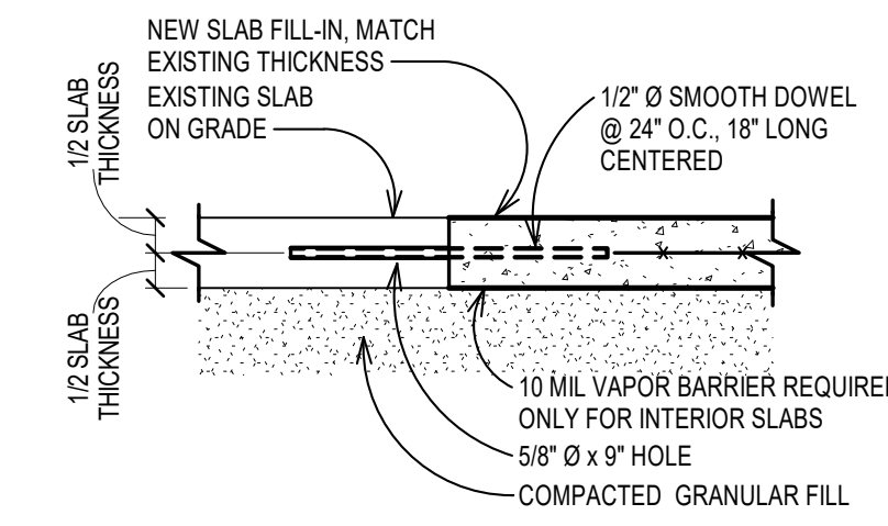
5 SLAB REPAIR DETAIL SCALE: 1" = 1'-0"
