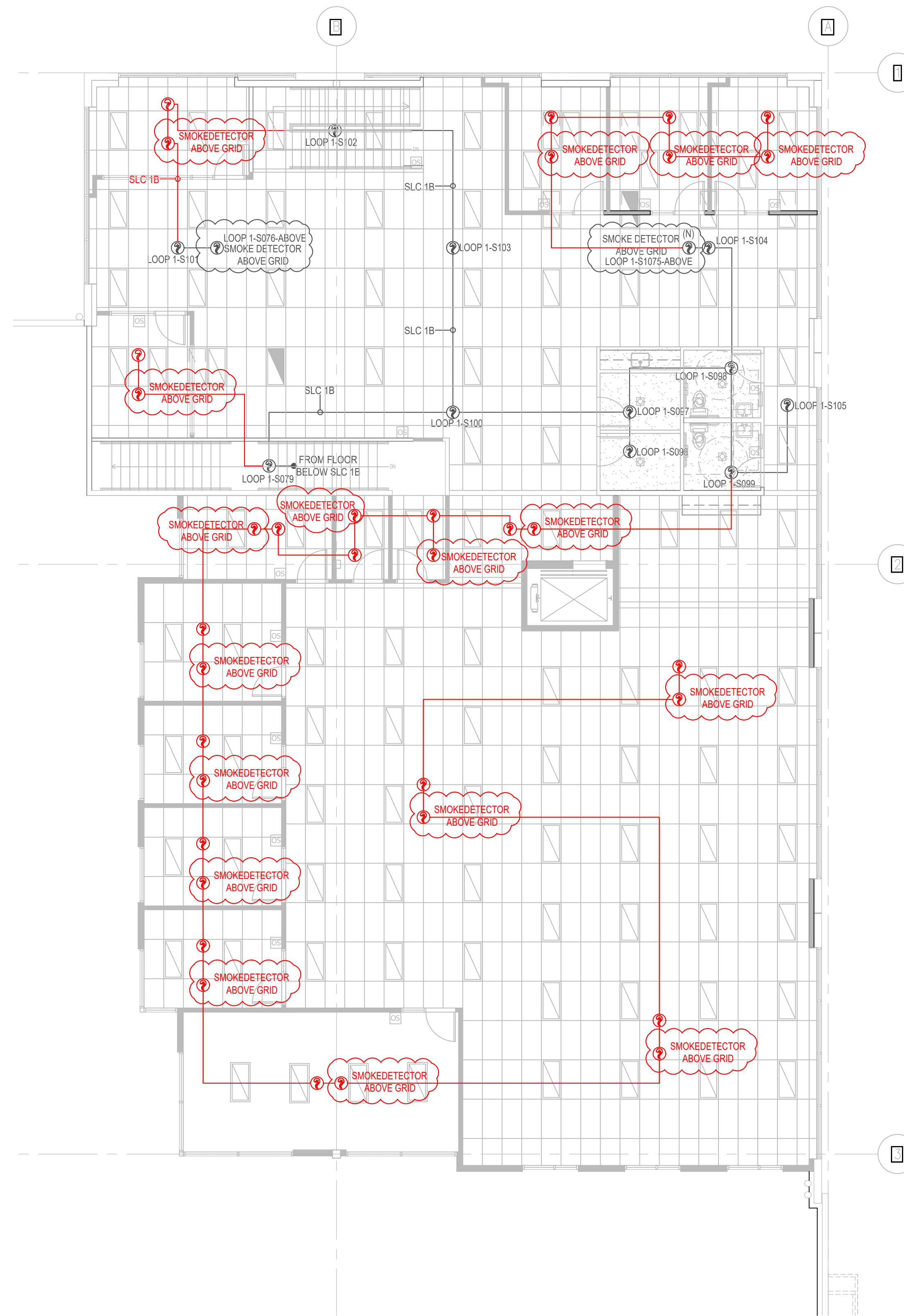
FIRE ALARM OFFICE 2ND FLOOR SMOKE DETECTOR LAYOUT 1/8"=1'-0"
