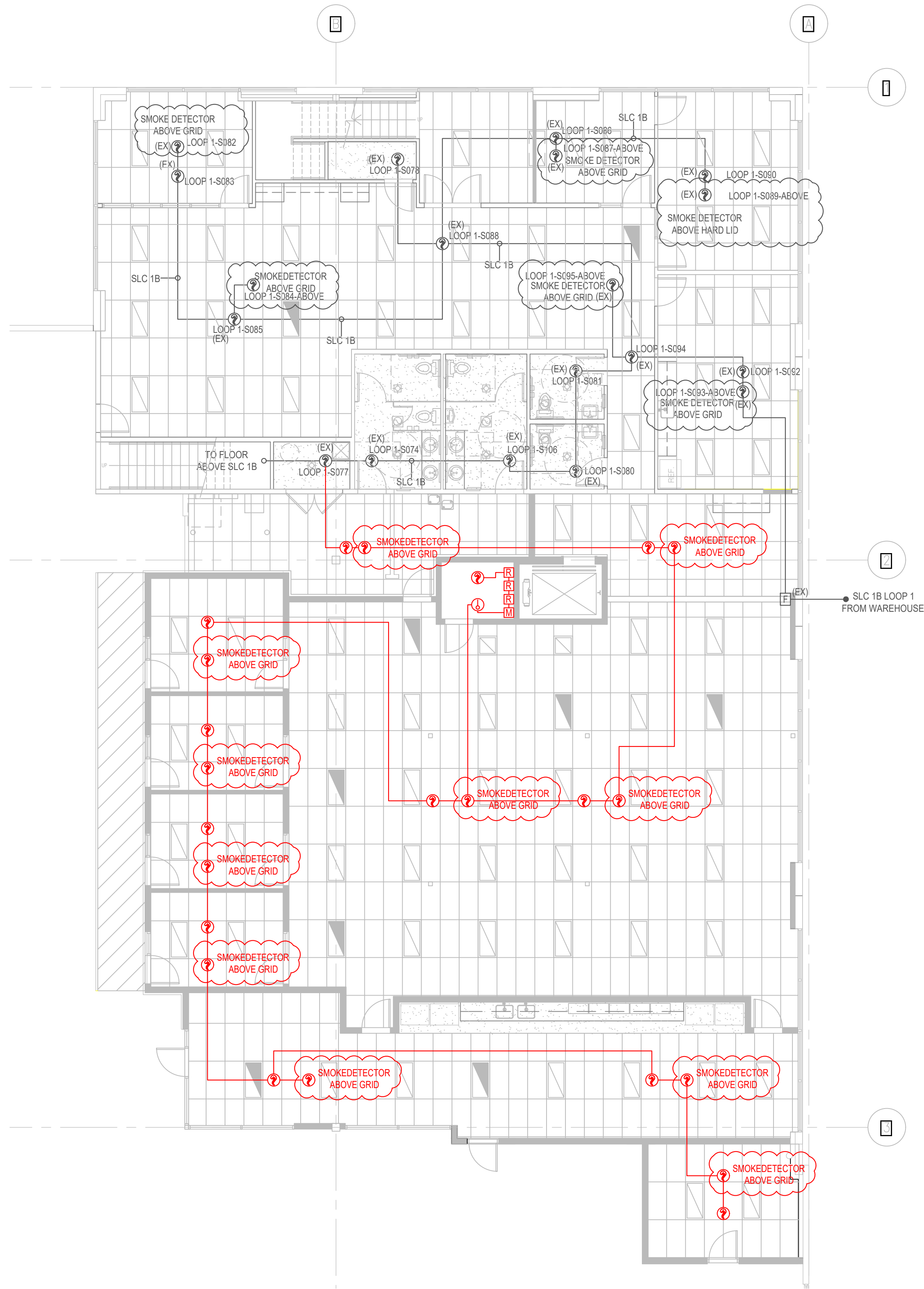
FIRE ALARM OFFICE 1ST FLOOR SMOKE DETECTOR LAYOUT 1/8"=1'-0"
