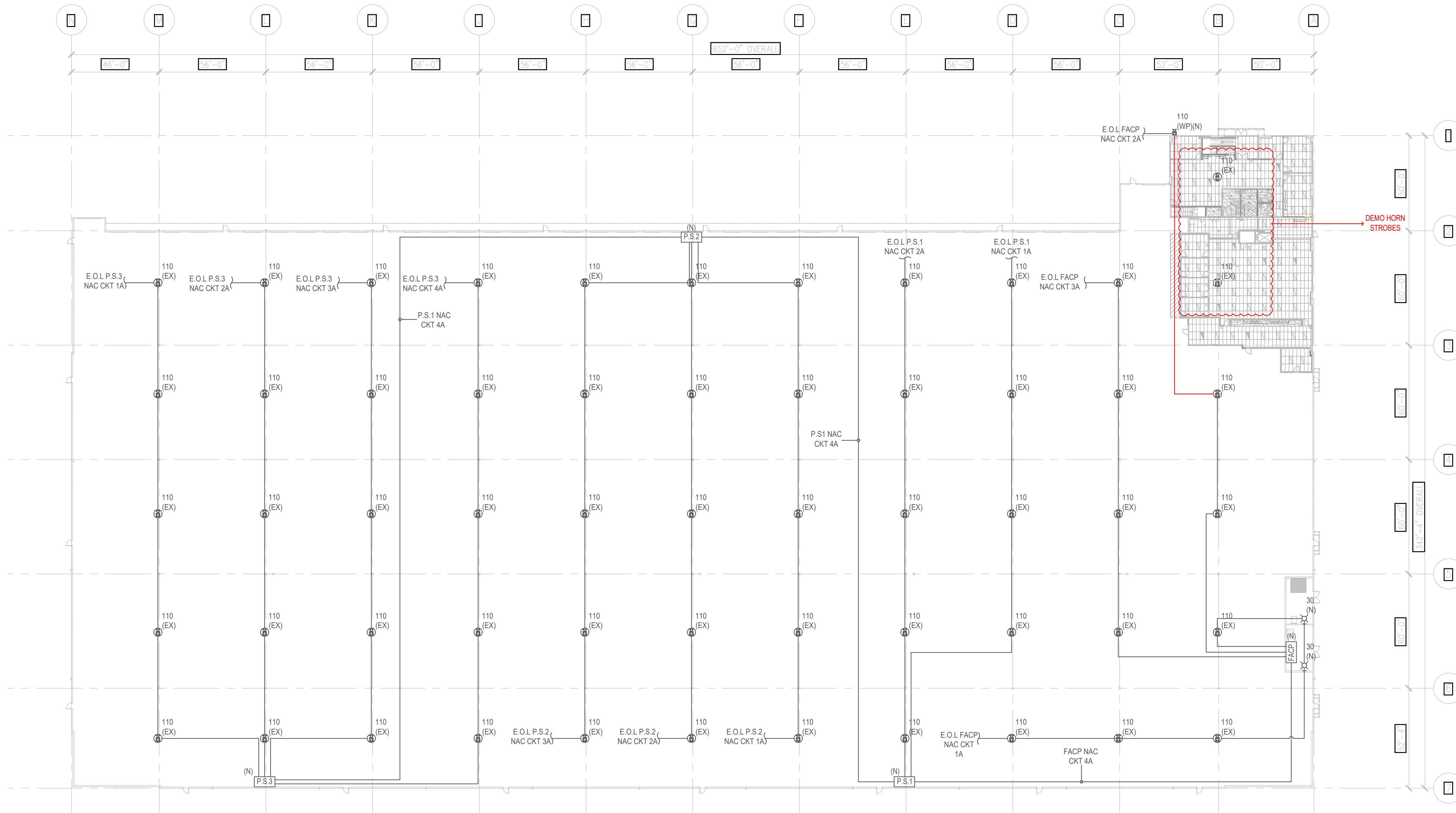
FIRE ALARM WAREHOUSE NAC LAYOUT 1/32" = 1'-0"
