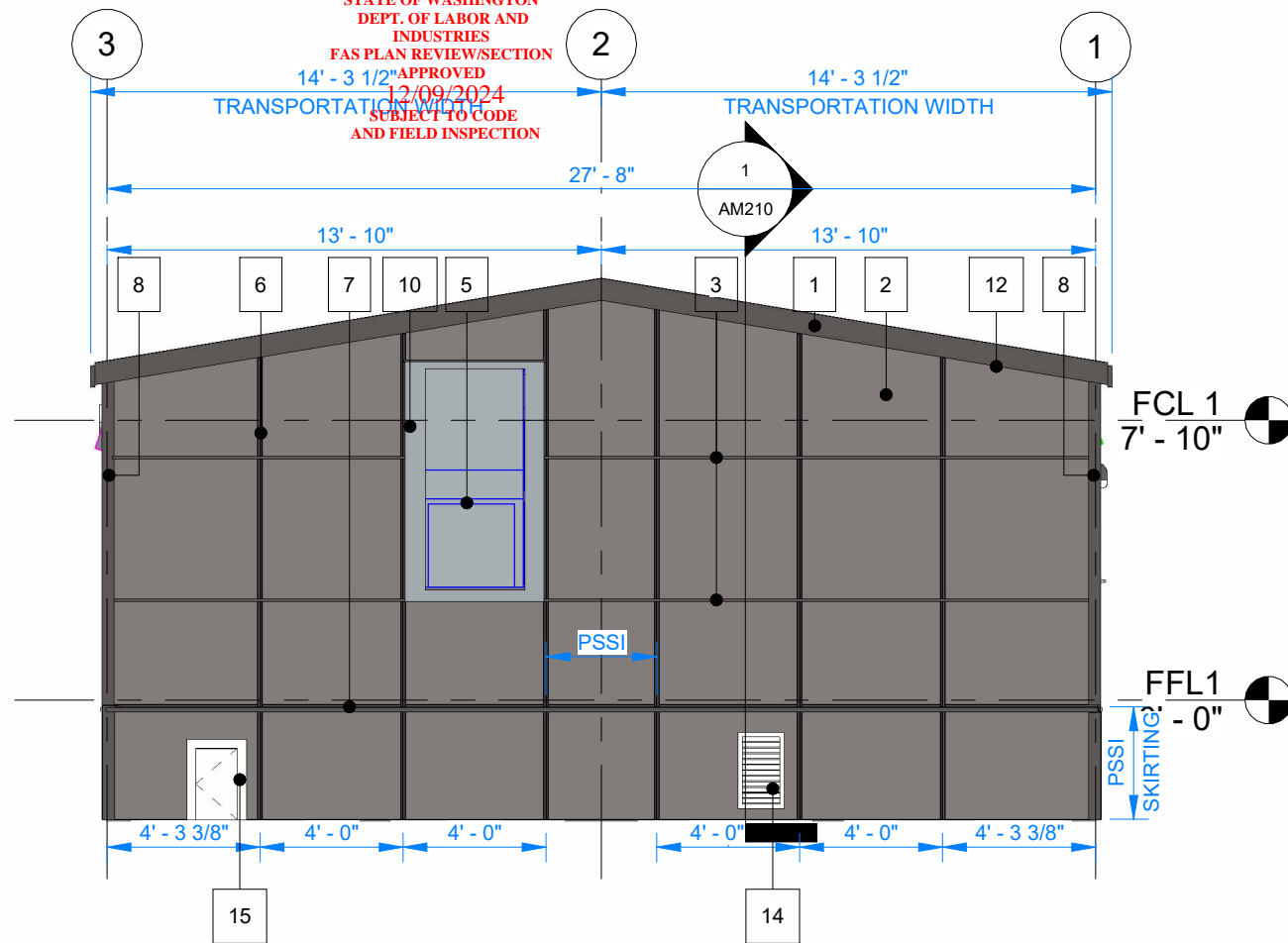
1 RIGHT ELEVATION 3/16" = 1'-0"
