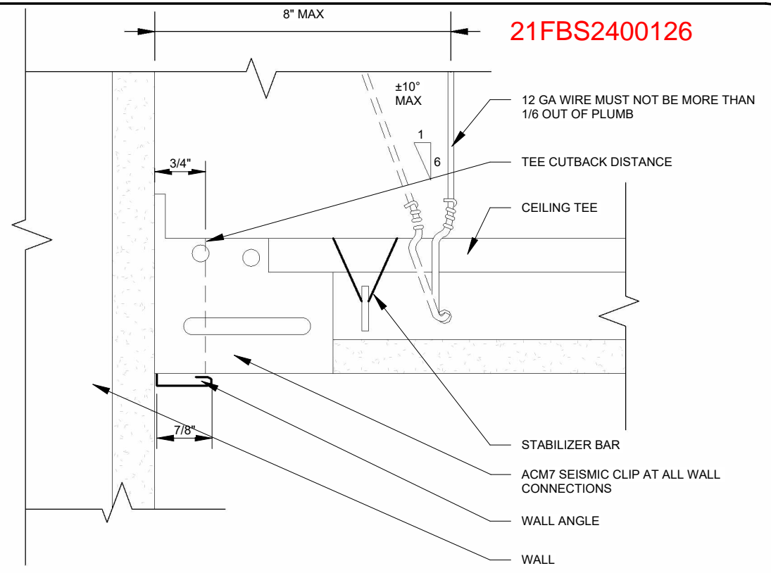
3 SEISMIC ACT - DETACHED PERIMETER DETAIL SCALE: 6" = 1'-0"
