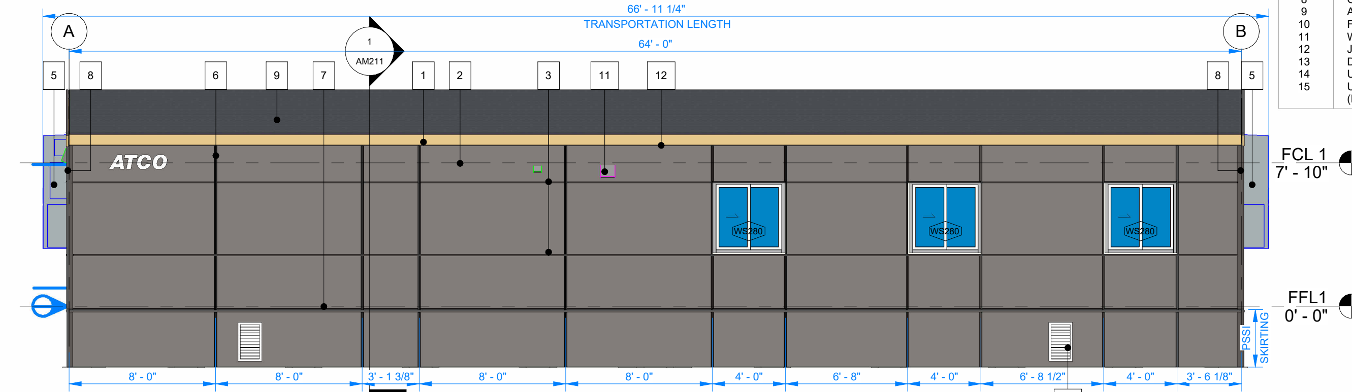
2 BACK ELEVATION 3/16" = 1'-0"
