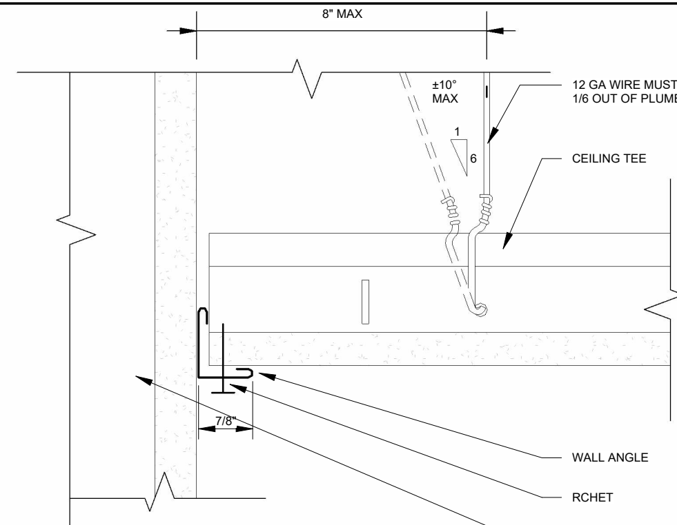
2 SEISMIC ACT - ATTACHED PERIMETER DETAIL SCALE: 6" = 1'-0"
