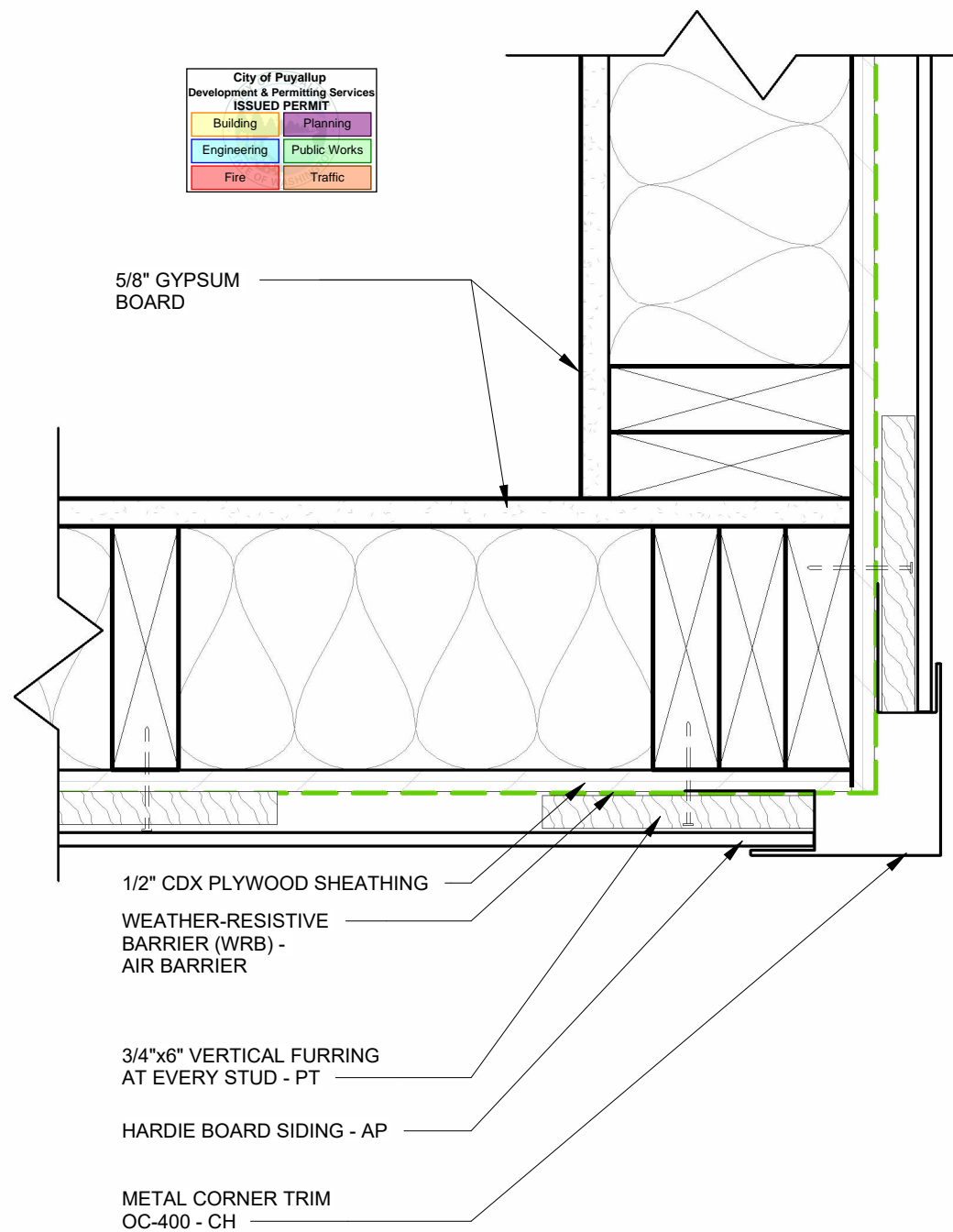
1 HARDIE BOARD SIDING CORNER1 3" = 1'-0"
