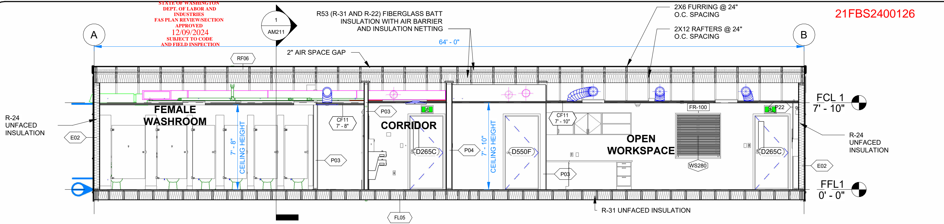
1 BUILDING SECTION - LONG 3/16" = 1'-0"
