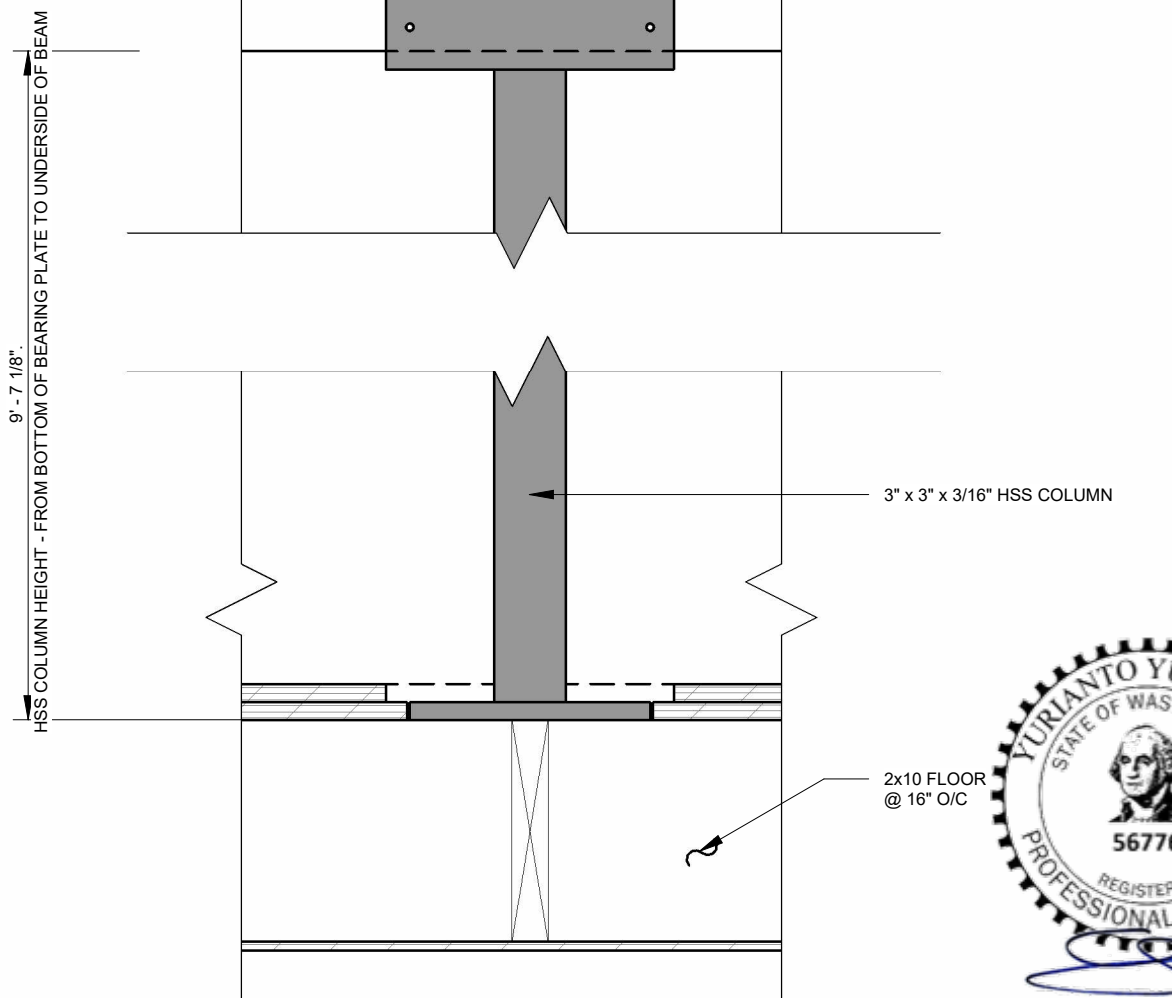
3 HSS COLUMN CONNECTION DETAIL SCALE: 1 1/2" = 1'-0"
