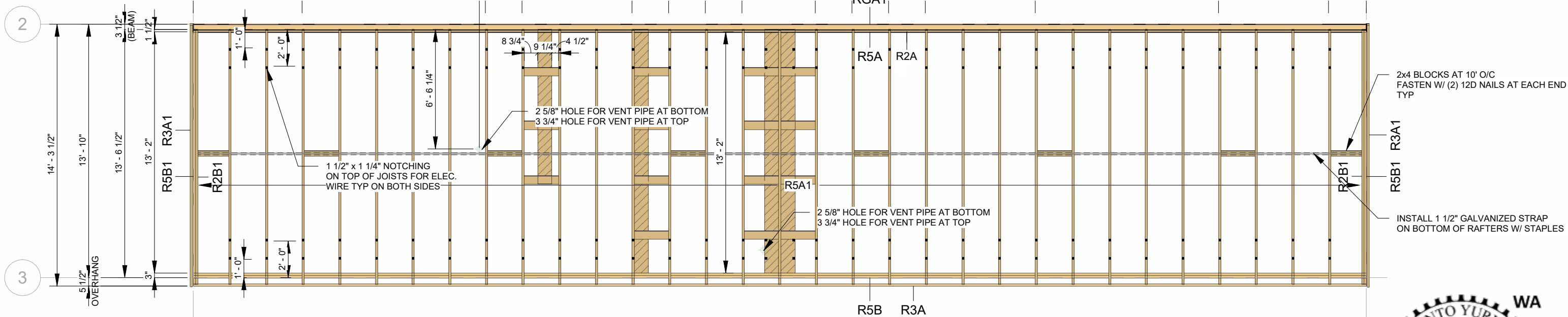
1 ROOF FRAMING - UNIT 102 AM200 SCALE: 3/16" = 1'-0"
