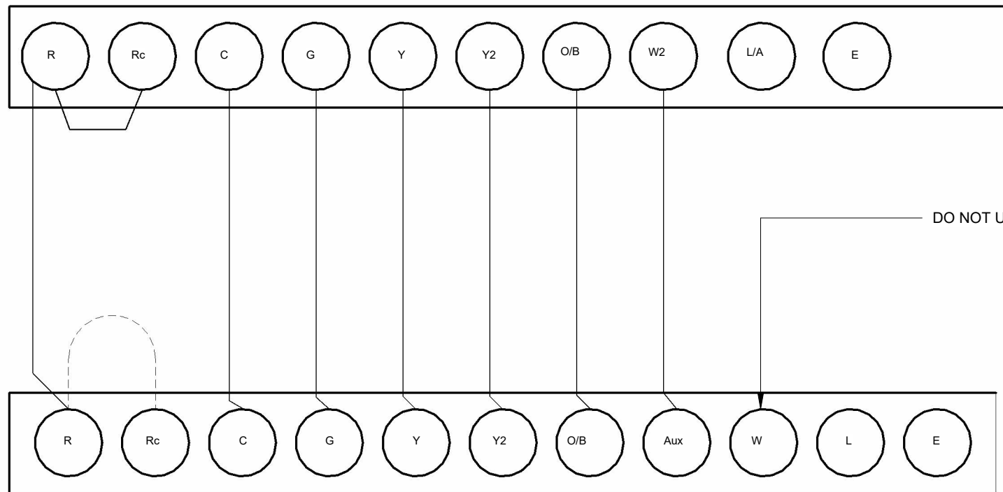
1 BARD CONNECTION 1/4" = 1'-0"
