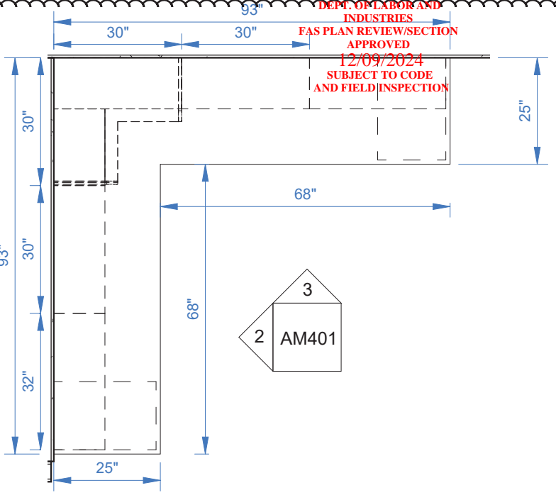
1 OPEN WORK SPACE MILLWORK 3/8" = 1'-0"
