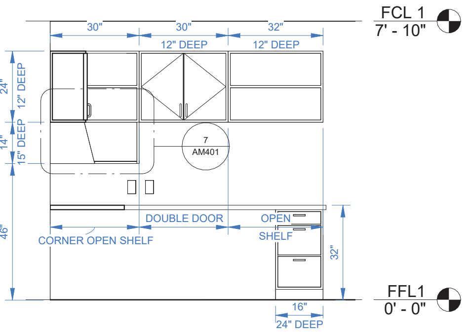
3 ELEVATION 2 3/8" = 1'-0"
