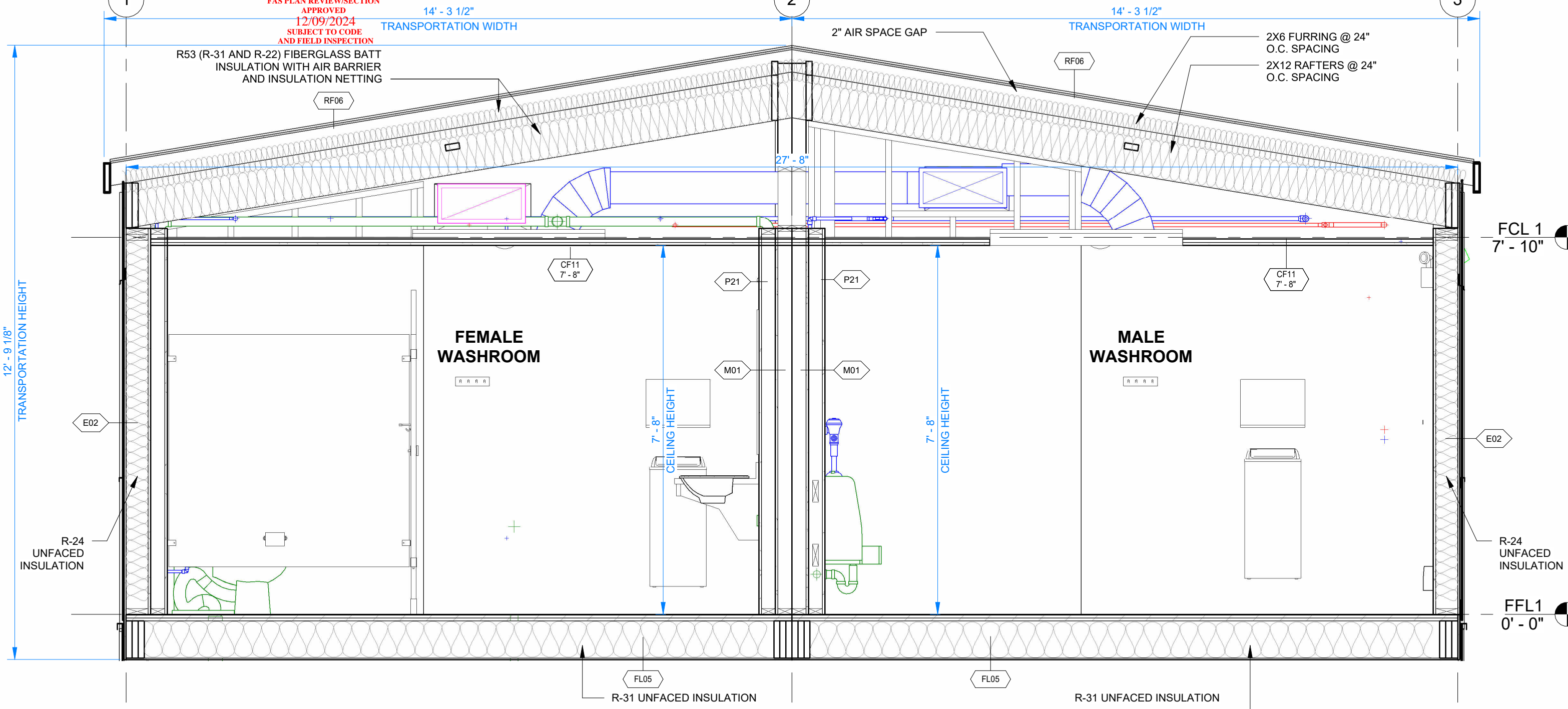
1 BUILDING SECTION - SHORT 1/2" = 1'-0"
