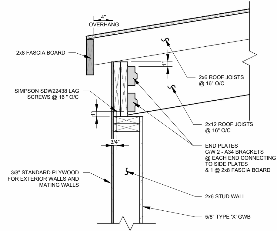
2 TYPICAL ROOF CONNECTION DETAIL @ LONG WALL SCALE: 1" = 1'-0"
