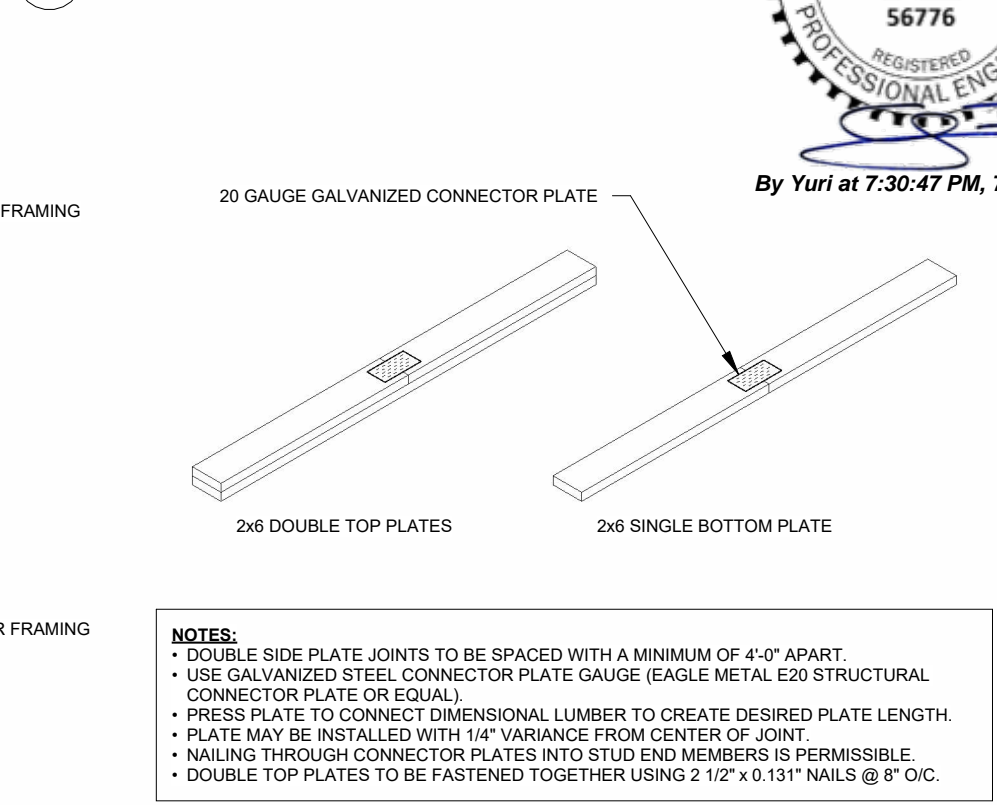
5 TYPICAL LUMBER CONNECTION DETAIL
