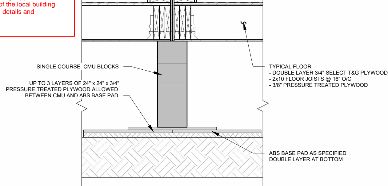
2 FOUNDATION MATING LINE DETAIL
