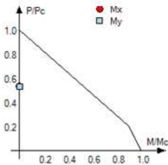
INTERACTION DIAGRAM
