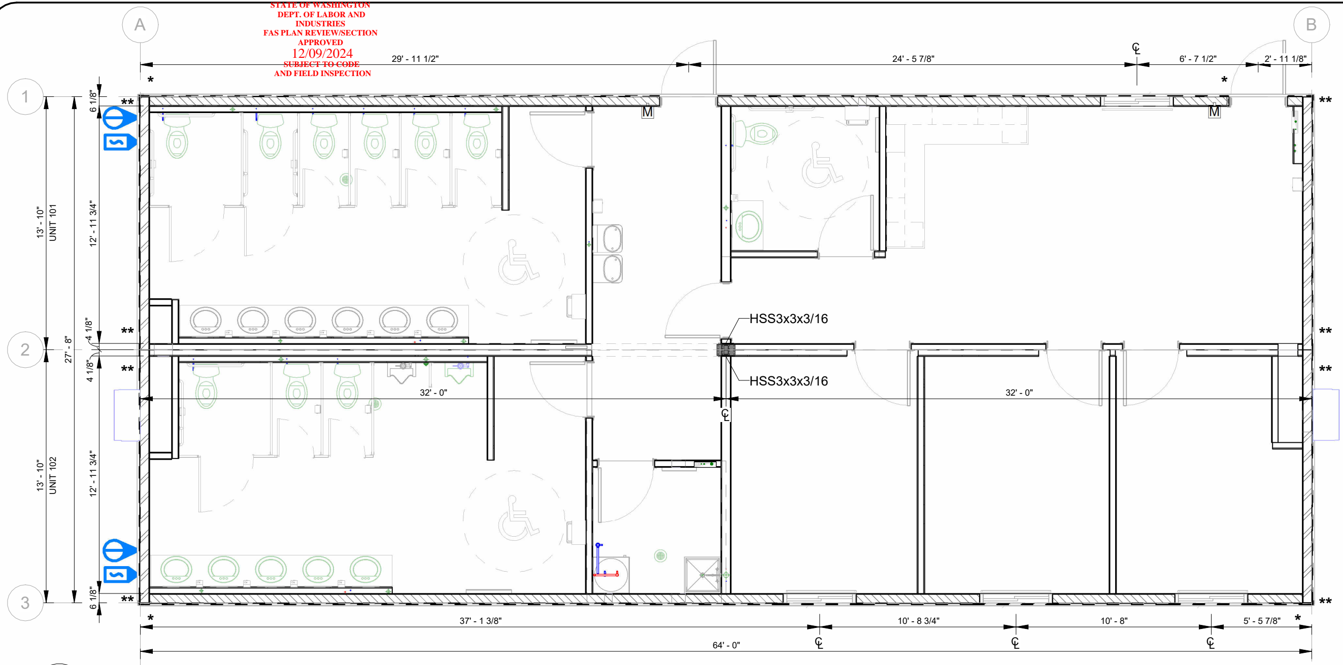
1 OVERALL STRUCTURAL FLOOR PLAN AM200 SCALE: 3/16" = 1'-0"
