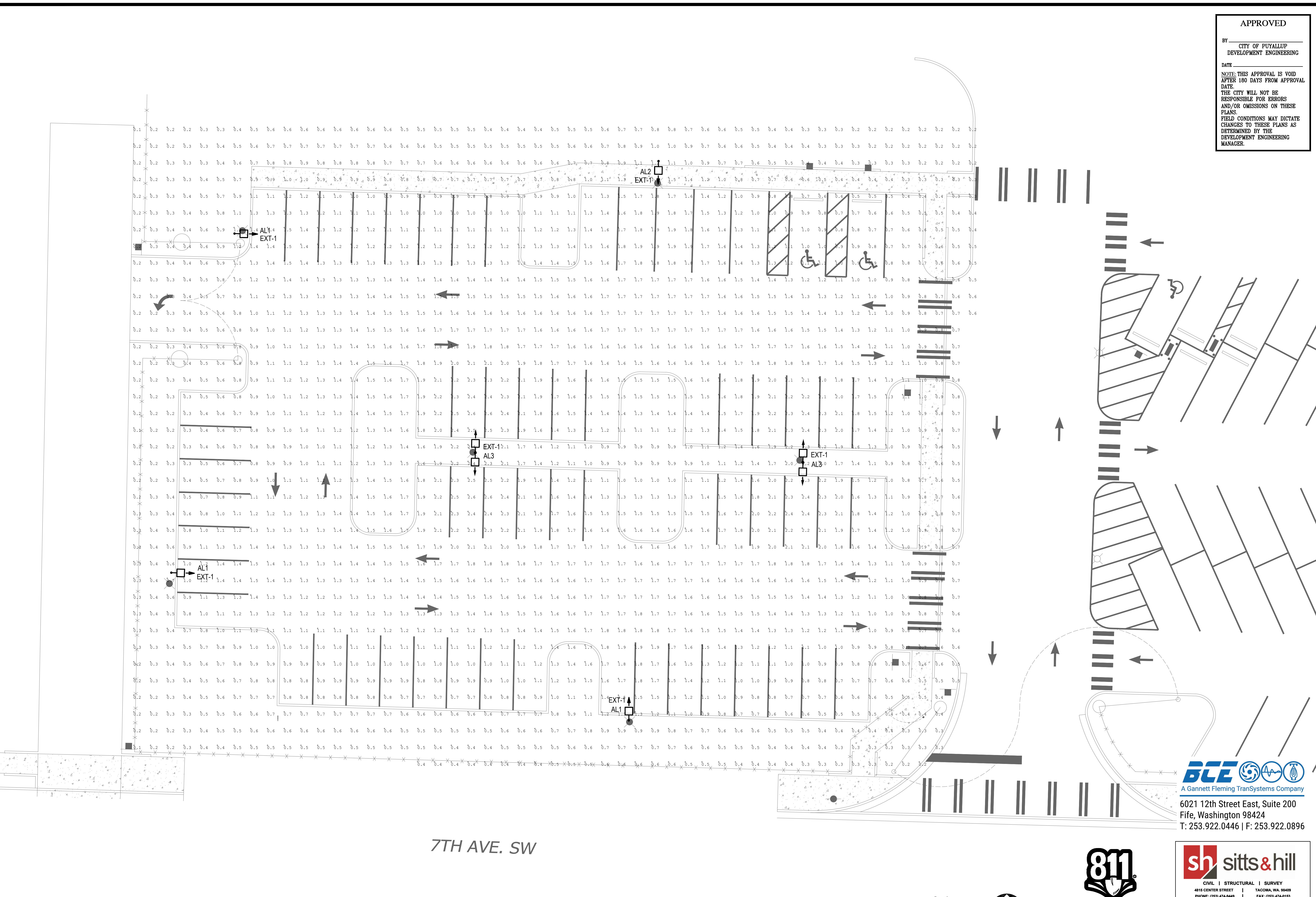
EVENT PARKING LAYOUT DESIGN OPTION 6 - LIGHTING CALCULATIONS SCALE: 1"=10'
