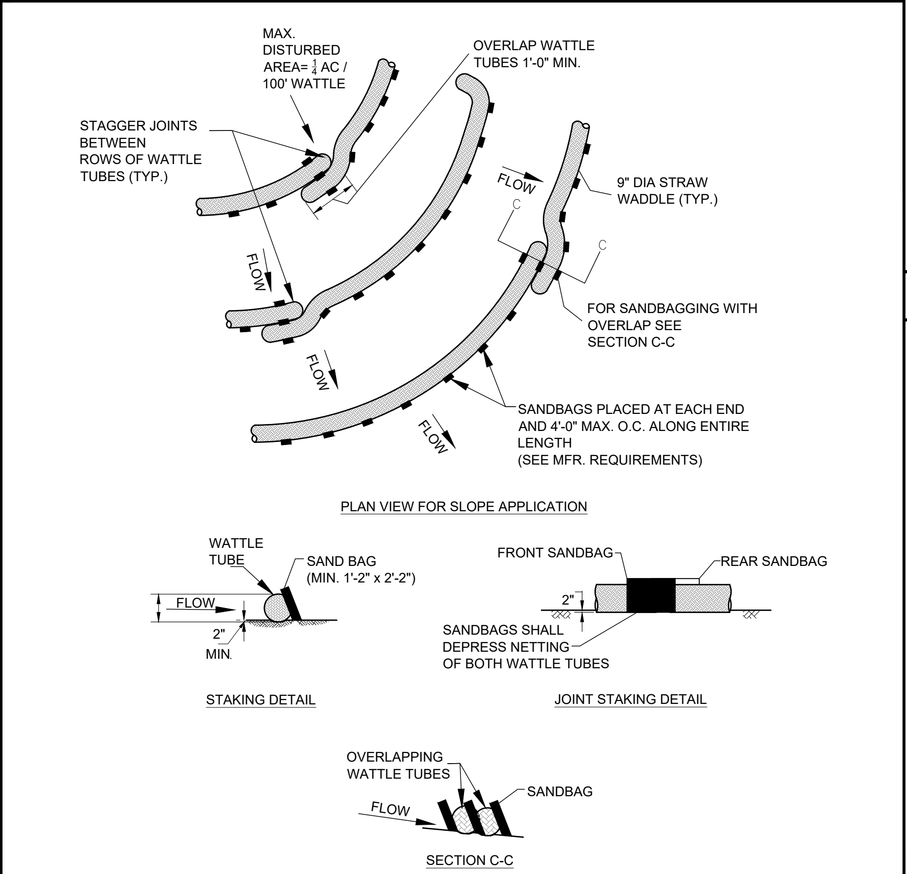
EROSION EEL / FILTER SOCK SCALE N.T.S. 6
