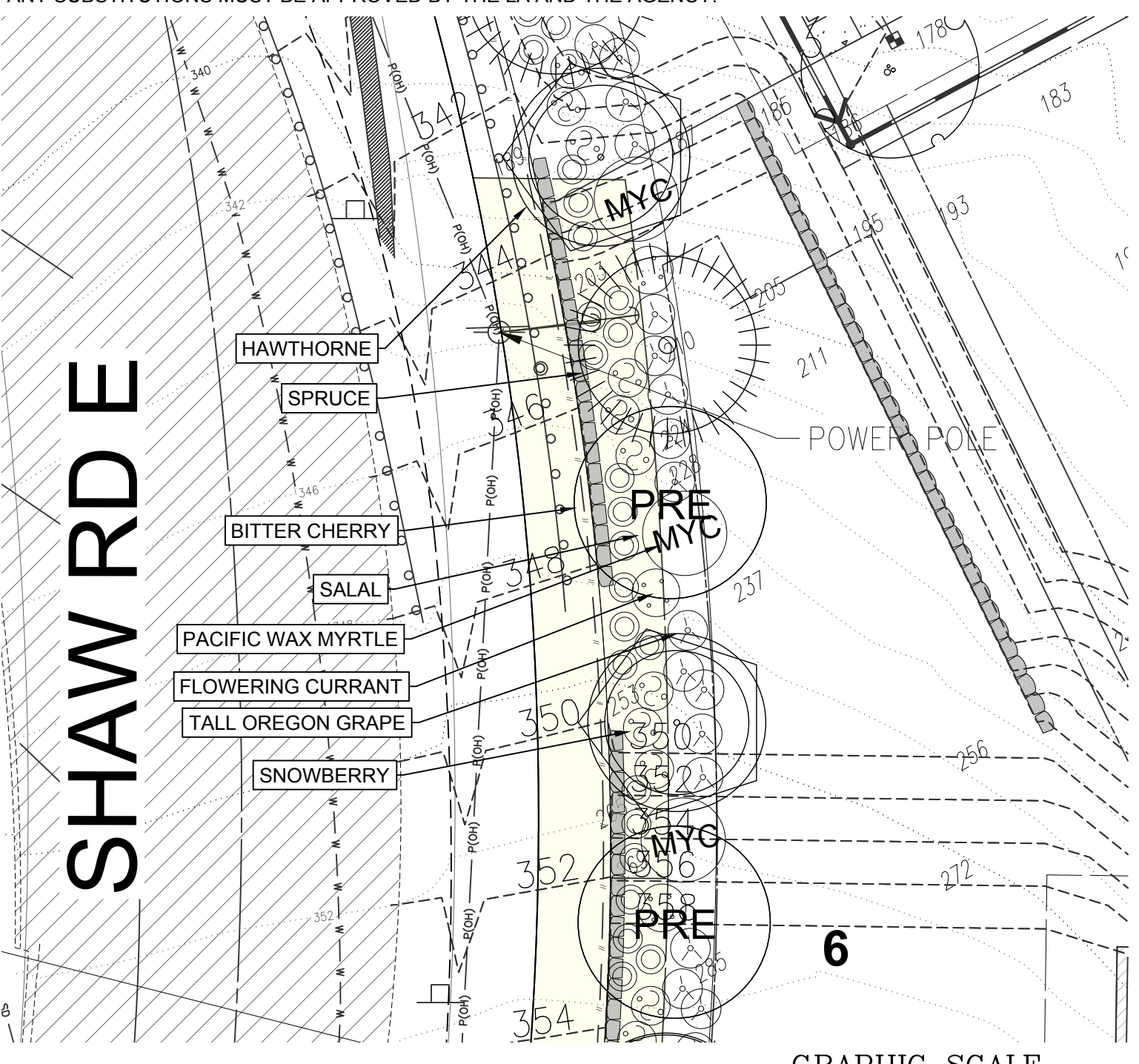
ENLARGED TYPE II PERIMETER PLANTING PLAN ( IN FEET ) 1 inch = 20 ft.
