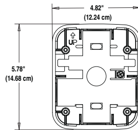
Surface Mount Back Box for Walls (SBBRL/SBBWL)
