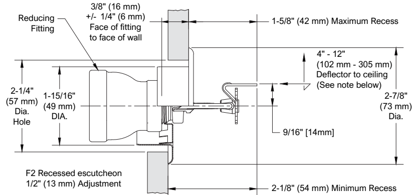
Models F1 & F1FR Horizontal Sidewall Sprinkler with Model F2 Recessed Escutcheon 1/2" (13mm) Nominal Adjustment (Note: Deflector distance is 4" to 6" (100 to 150 mm) for FM installations.)
