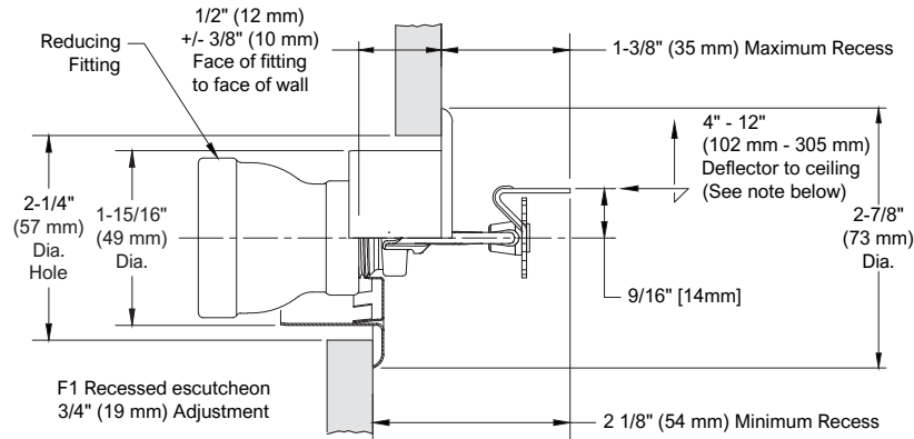
Models F1 & F1FR Horizontal Sidewall Sprinkler with Model F1 Recessed Escutcheon 3/4" (19mm) Nominal Adjustment (Note: Deflector distance is 4" to 6" (100 to 150 mm) for FM installations.)
