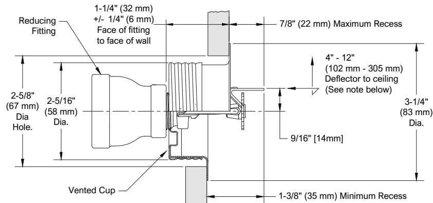
Models F1 & F1FR Horizontal Sidewall Sprinkler with Model FP Recessed Escutcheon 1/2" (13mm) Nominal Adjustment (Note: Deflector distance is 4" to 6" (100 to 150 mm) for FM installations.)
