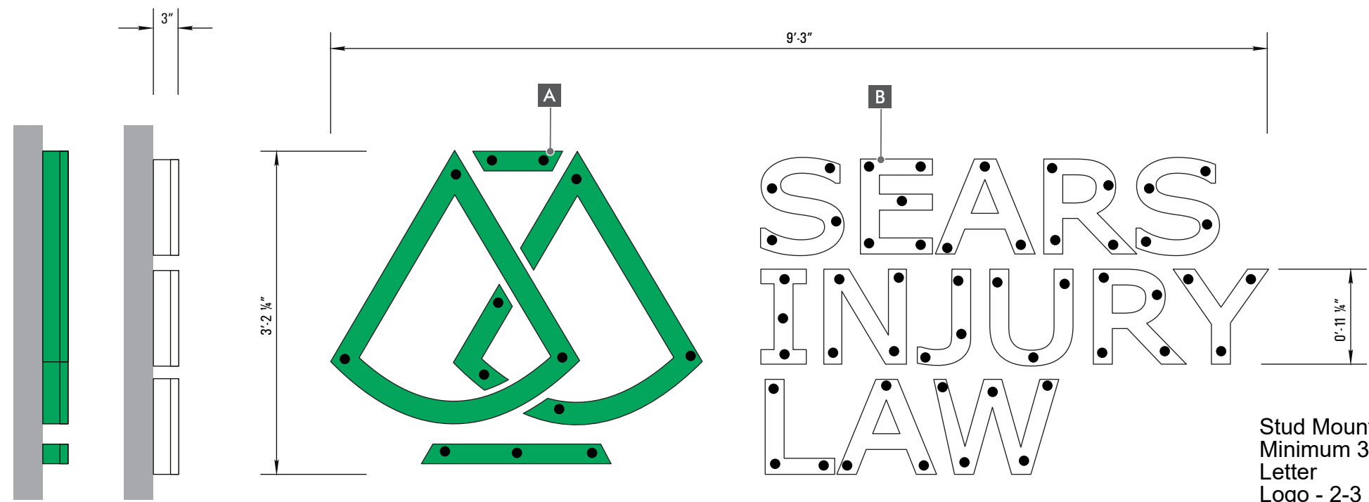
2 S/F ILLUMINATED DISPLAY WEST ELEVATION
