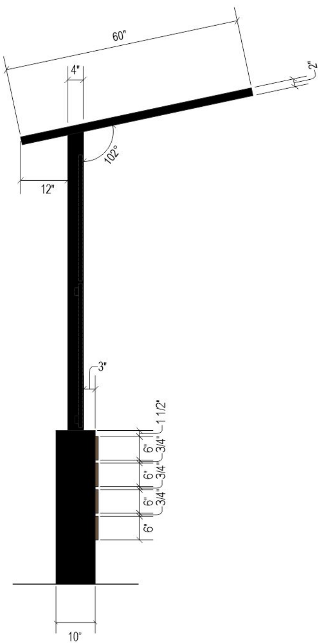
SIDE VIEW
