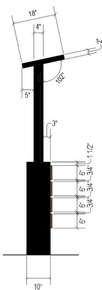
SIDE VIEW
