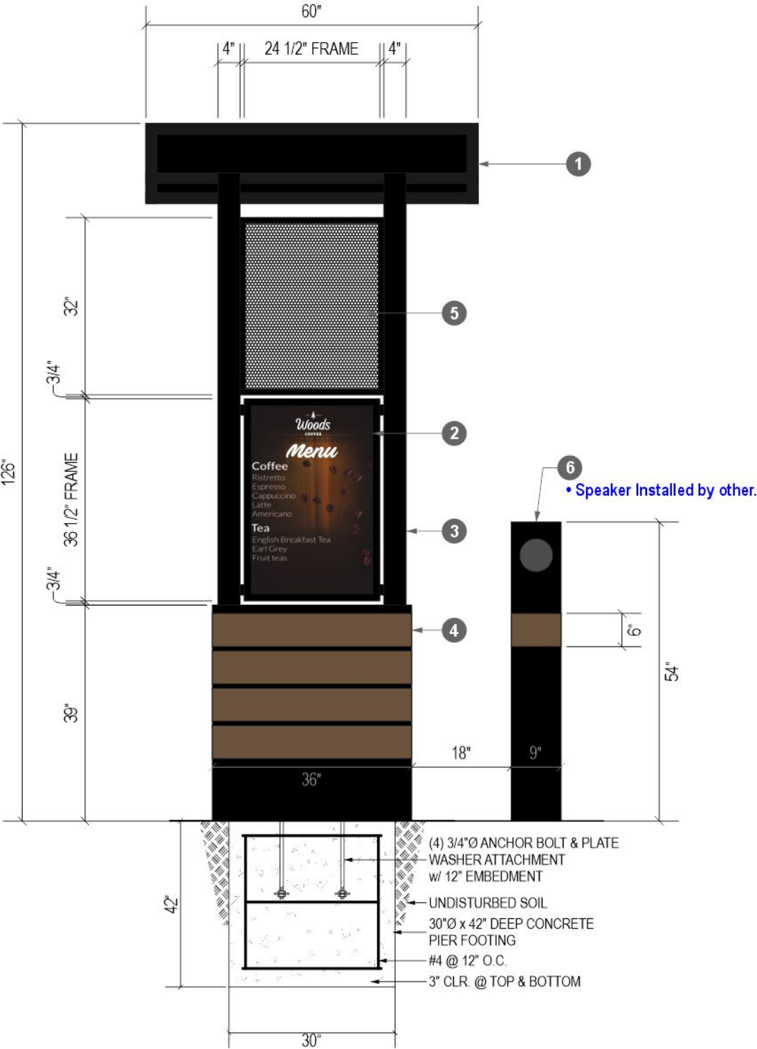
FRONT VIEW
