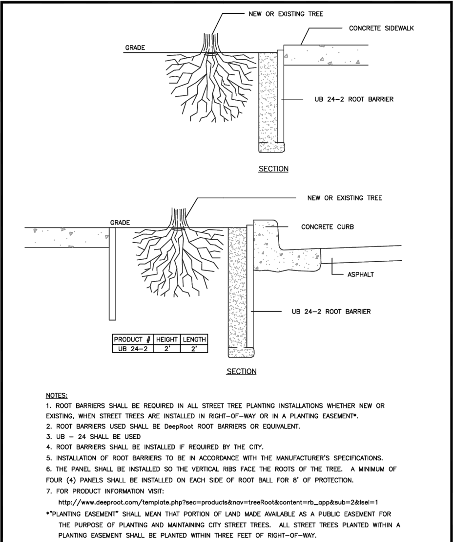
CITY OF PUYALLUP ROOT BARRIER DETAIL
