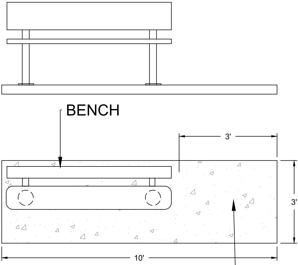
CONCRETE PAD W 3'X3' PAD FOR WHEELCHAIR 4" DEPTH MIN.
