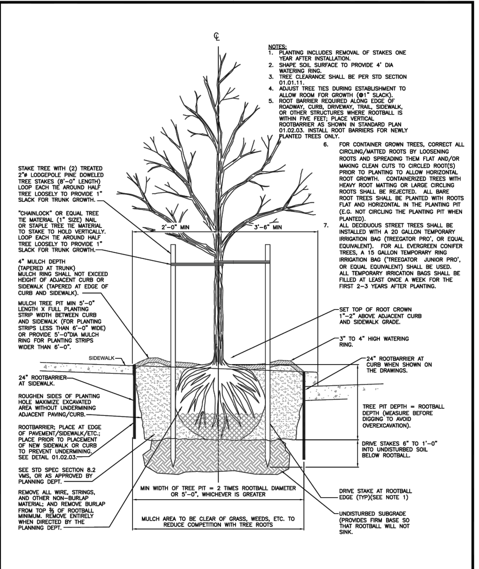
CITY OF PUYALLUP STREET TREE PLANTING IN PLANTING STRIP
