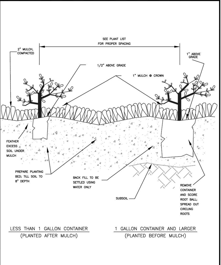
CITY OF PUYALLUP GROUND COVER PLANTING DETAIL
