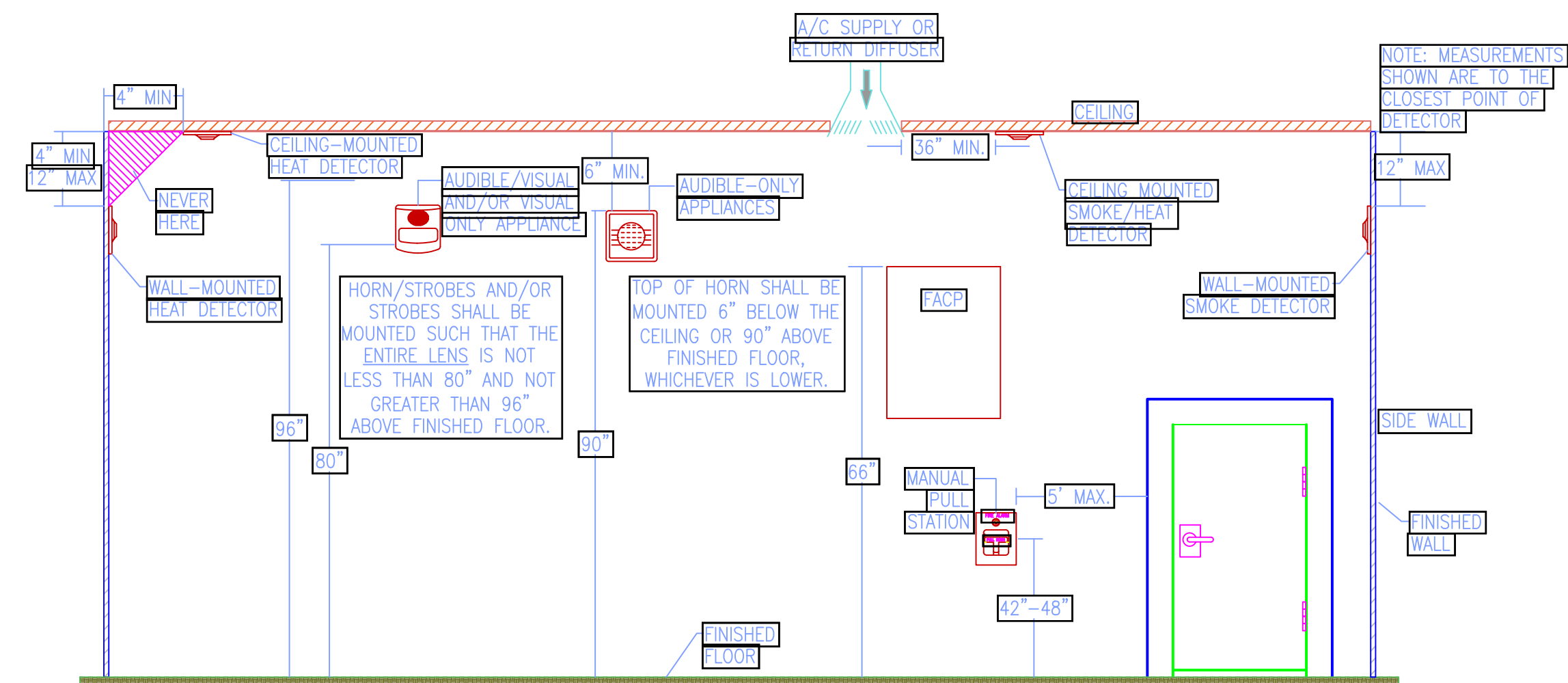
FIRE ALARM DEVICE MOUNTING HEIGHTS
