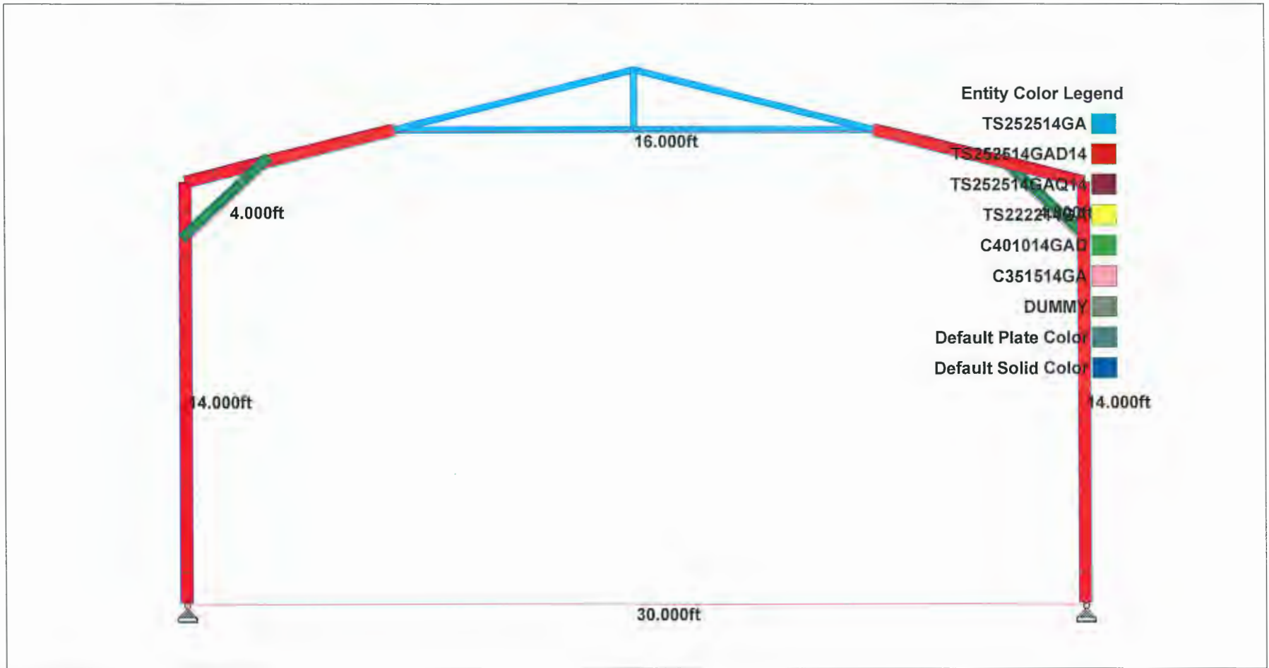
MAIN FRAME
