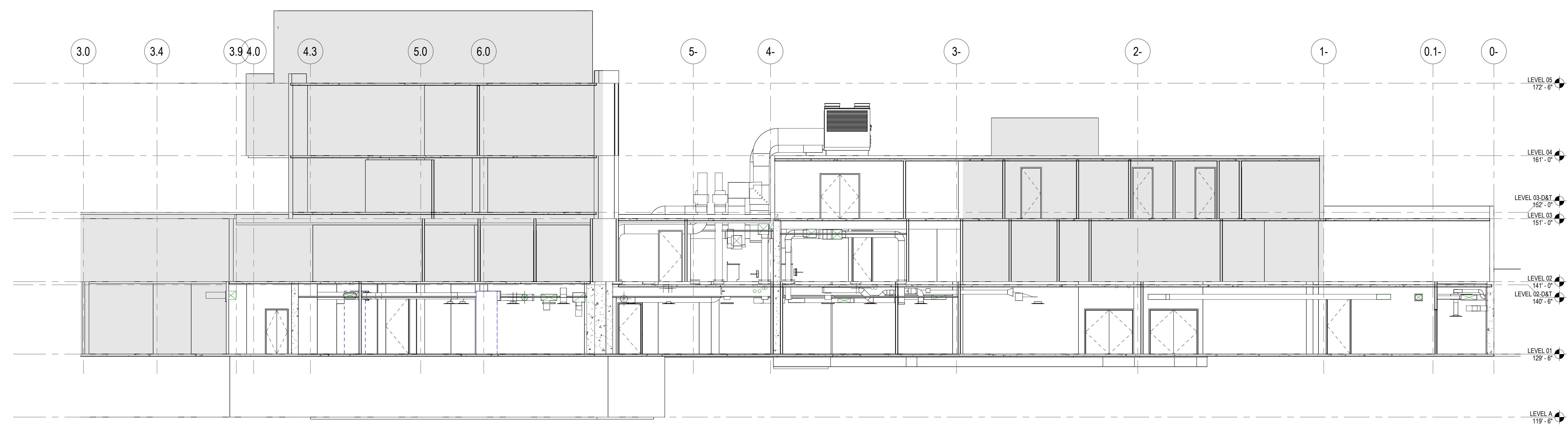
1 SITE SECTION E-W - SCALE 1/8" = 1'-0"
