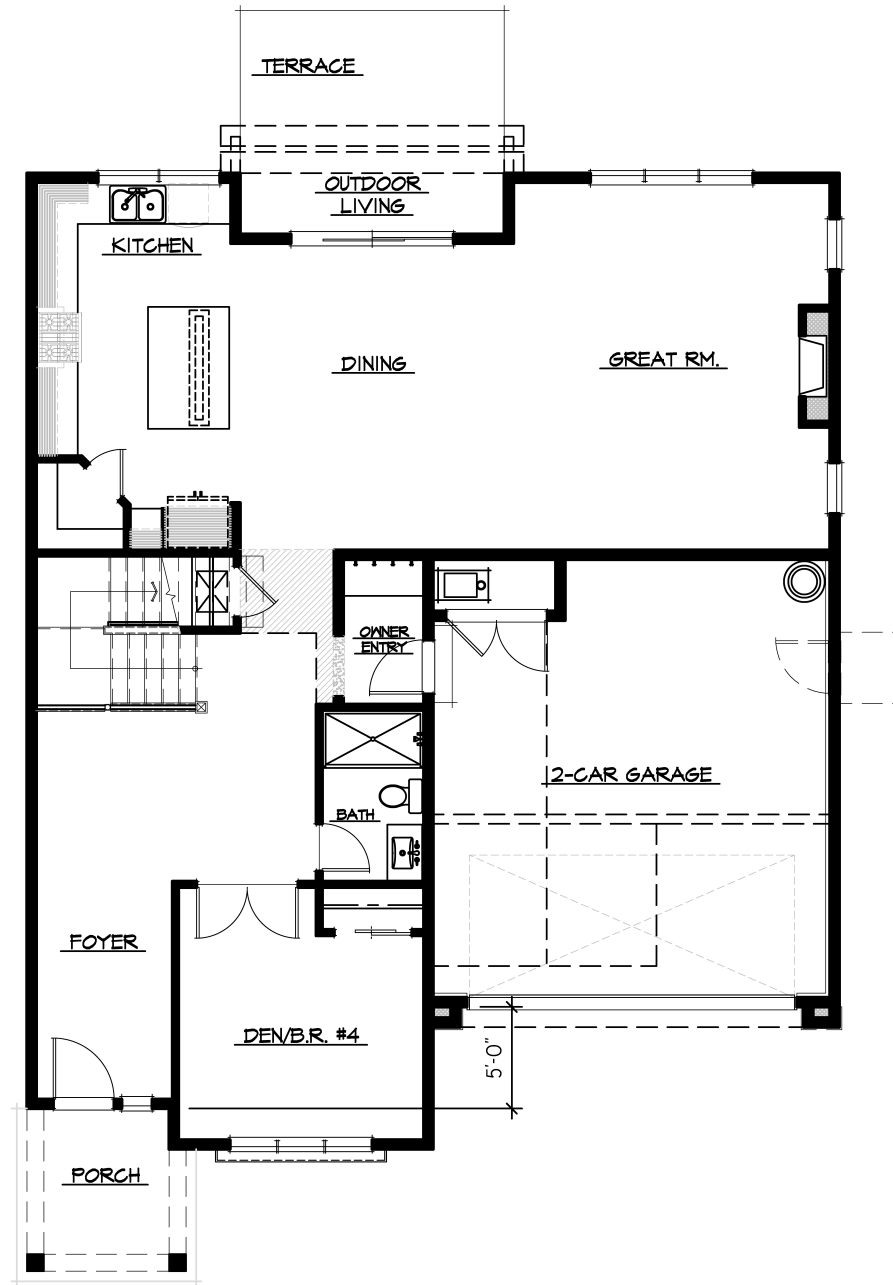
2600 DIMINISHED GARAGE FLOOR PLAN
