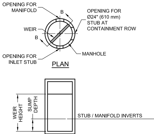
SECTION B-B DIVERSION MANHOLE DETAIL
