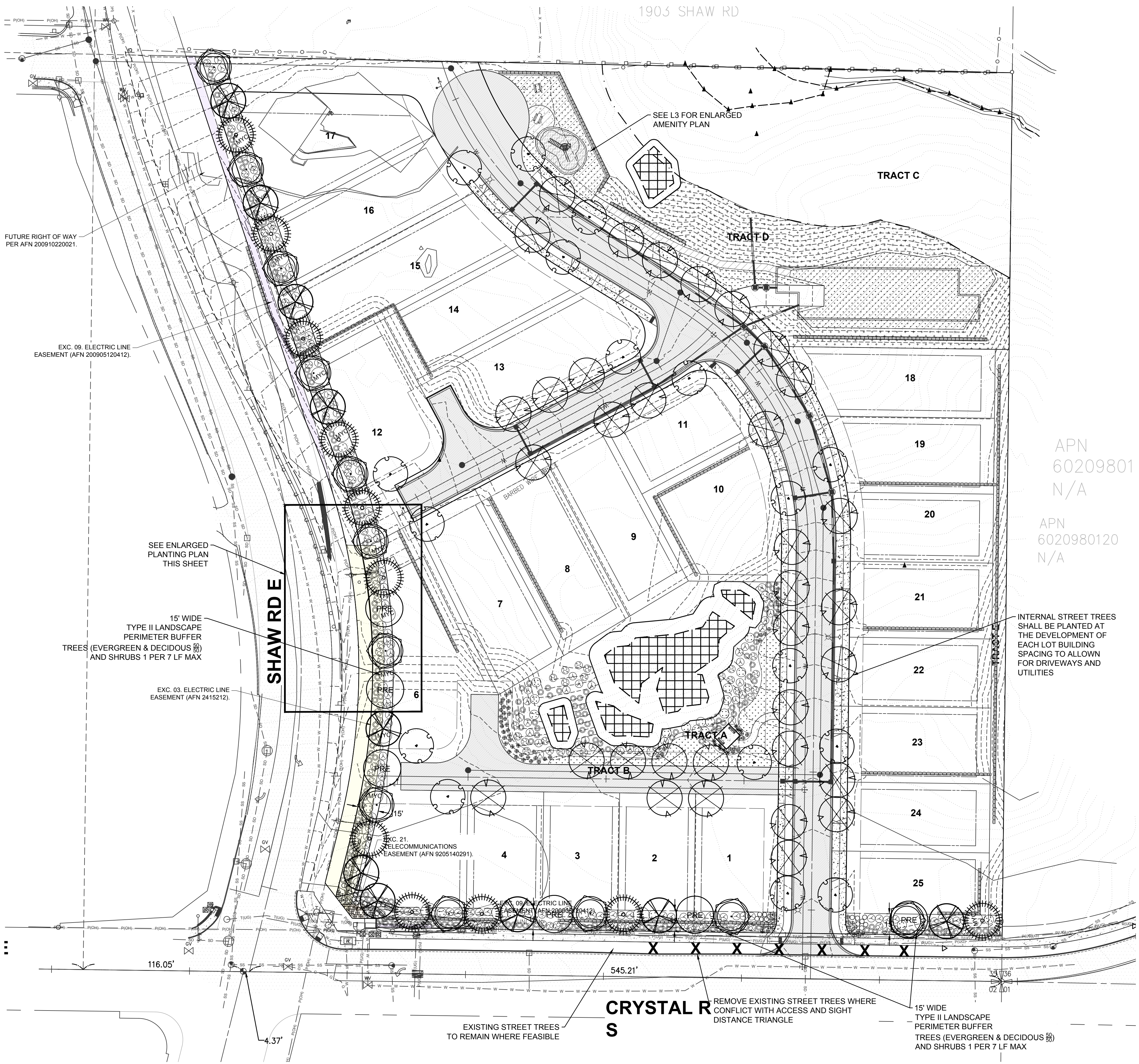
LANDSCAPE PLAN
