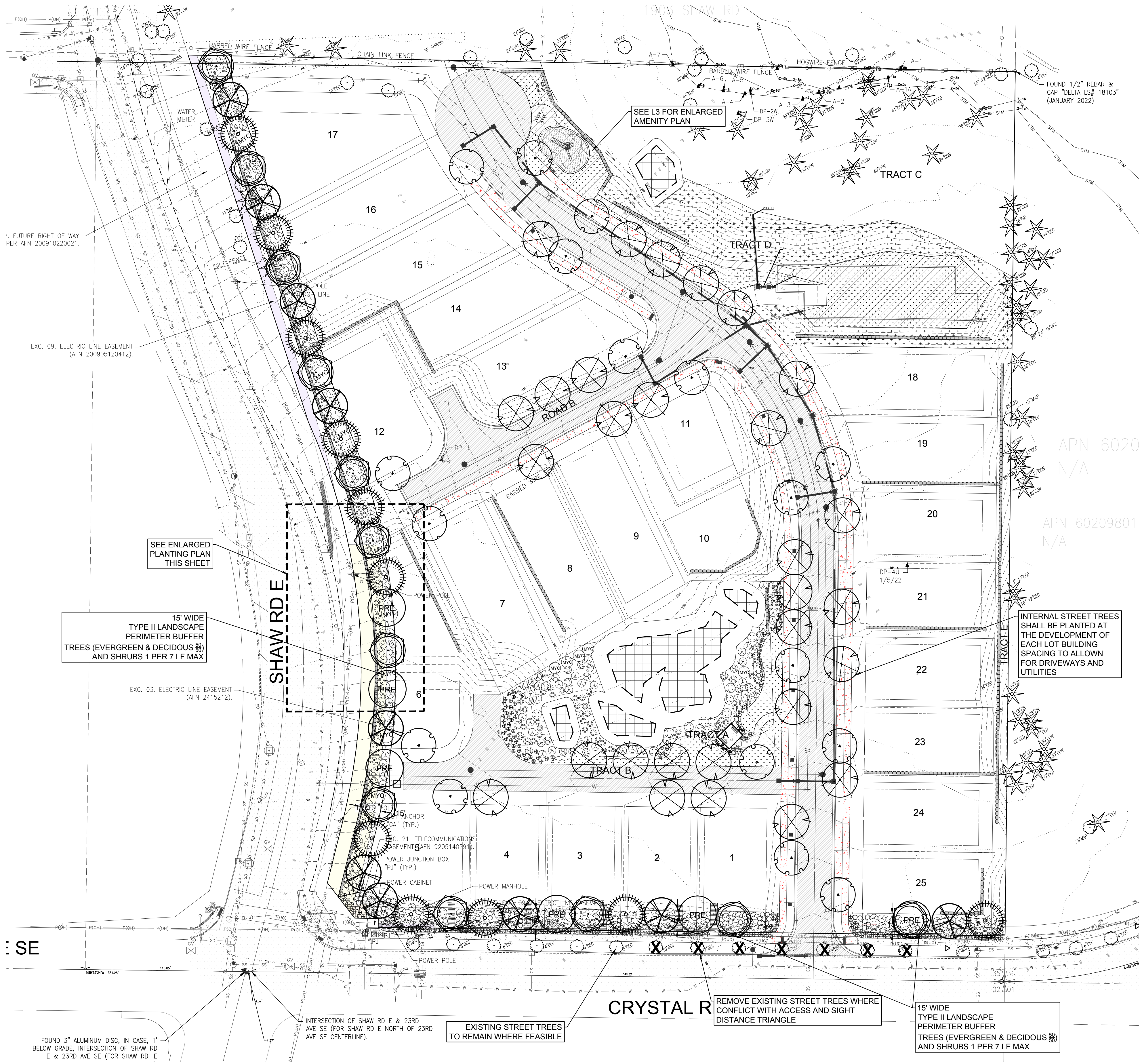
LANDSCAPE PLAN
