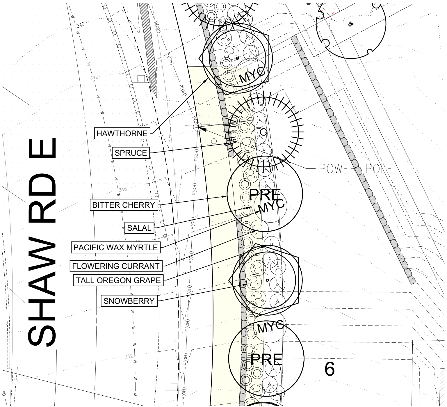
ENLARGED TYPE II PERIMETER PLANTING PLAN
