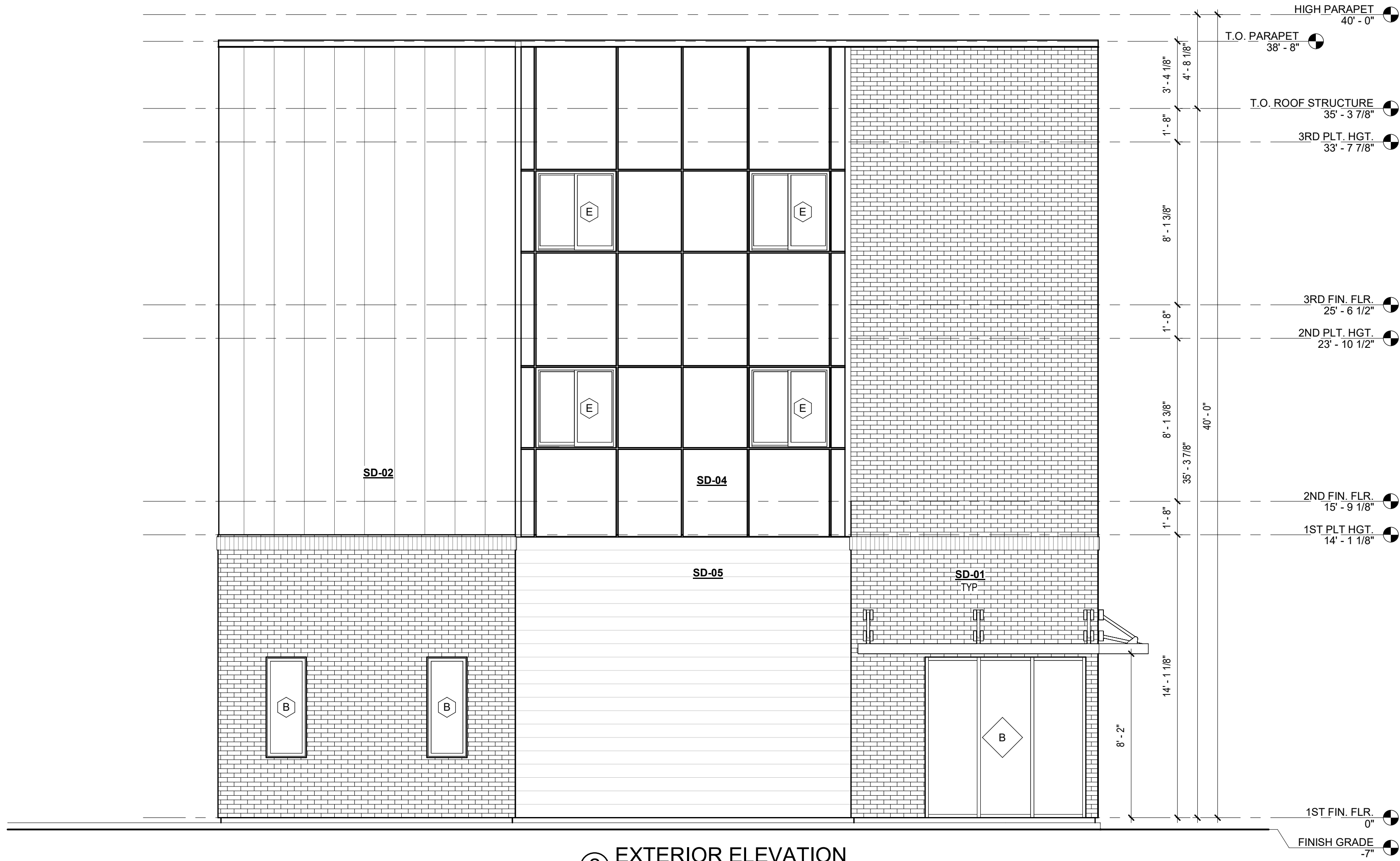
2 EXTERIOR ELEVATION 1/4" = 1'-0"
