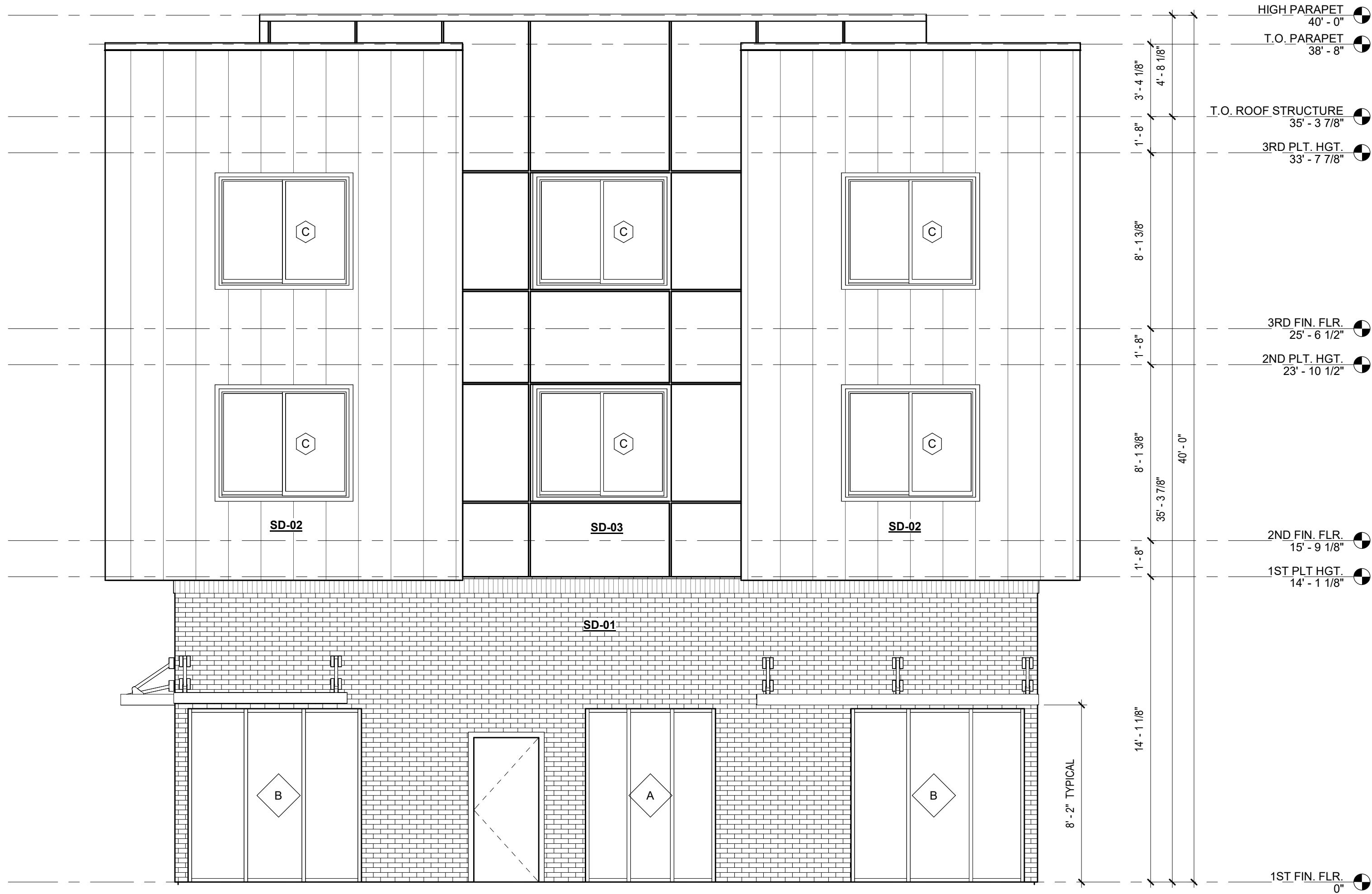
2 EXTERIOR ELEVATION 1/4" = 1'-0"
