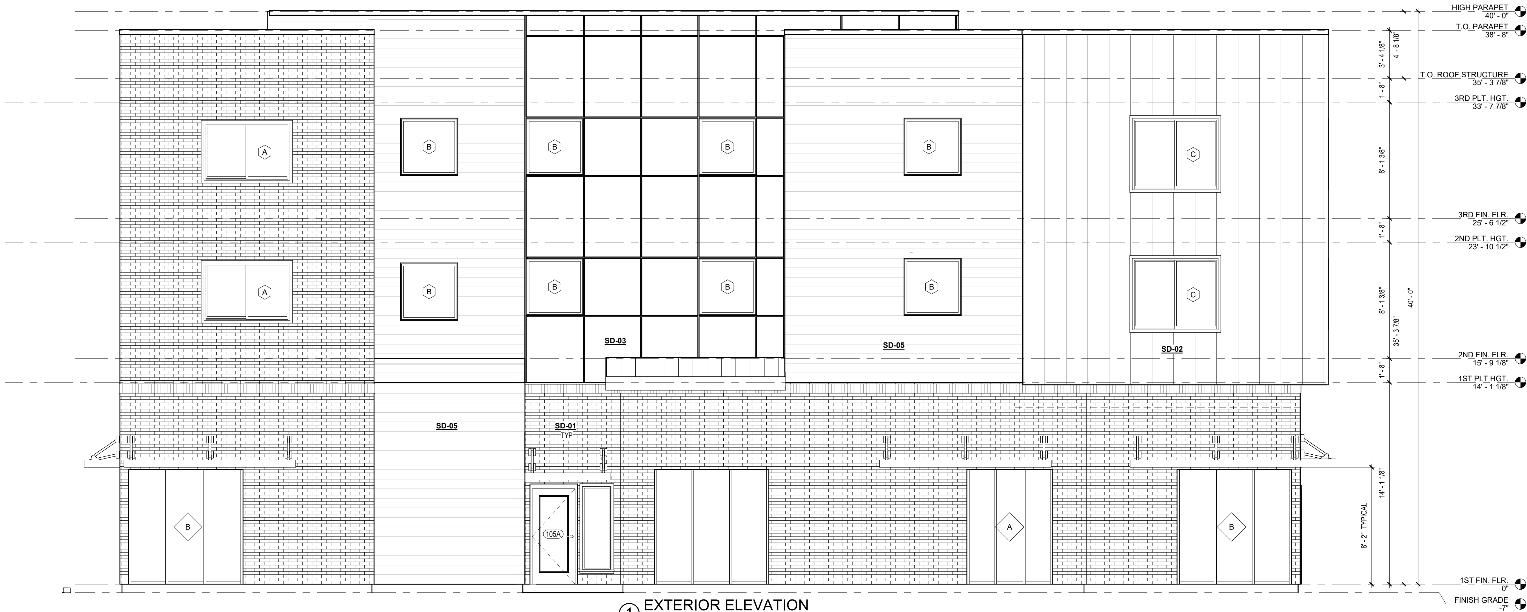
1 EXTERIOR ELEVATION 1/4" = 1'-0"
