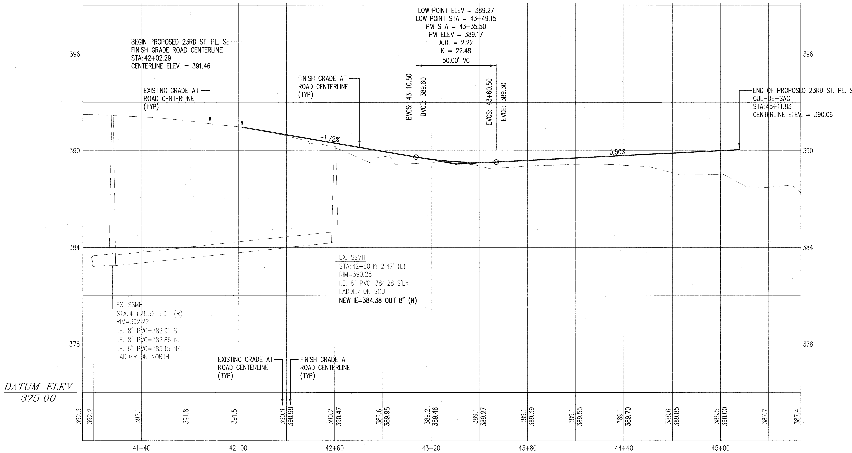
23RD ST PL SE HORIZONTAL: 1"=30' VERTICAL: 1"=3'
