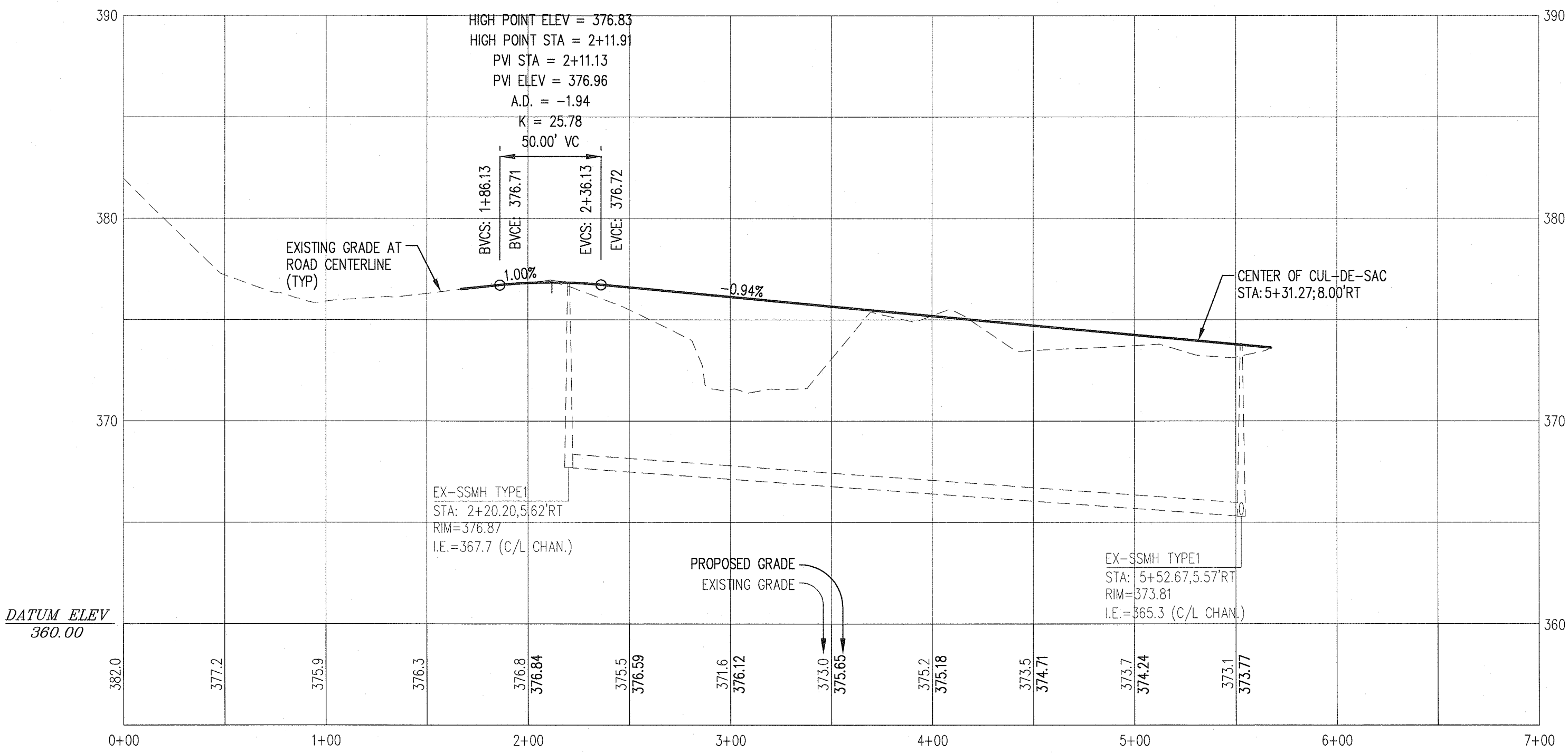
19TH AVE SE/TRACT C HORIZONTAL: 1"=50' VERTICAL: 1"=5'
