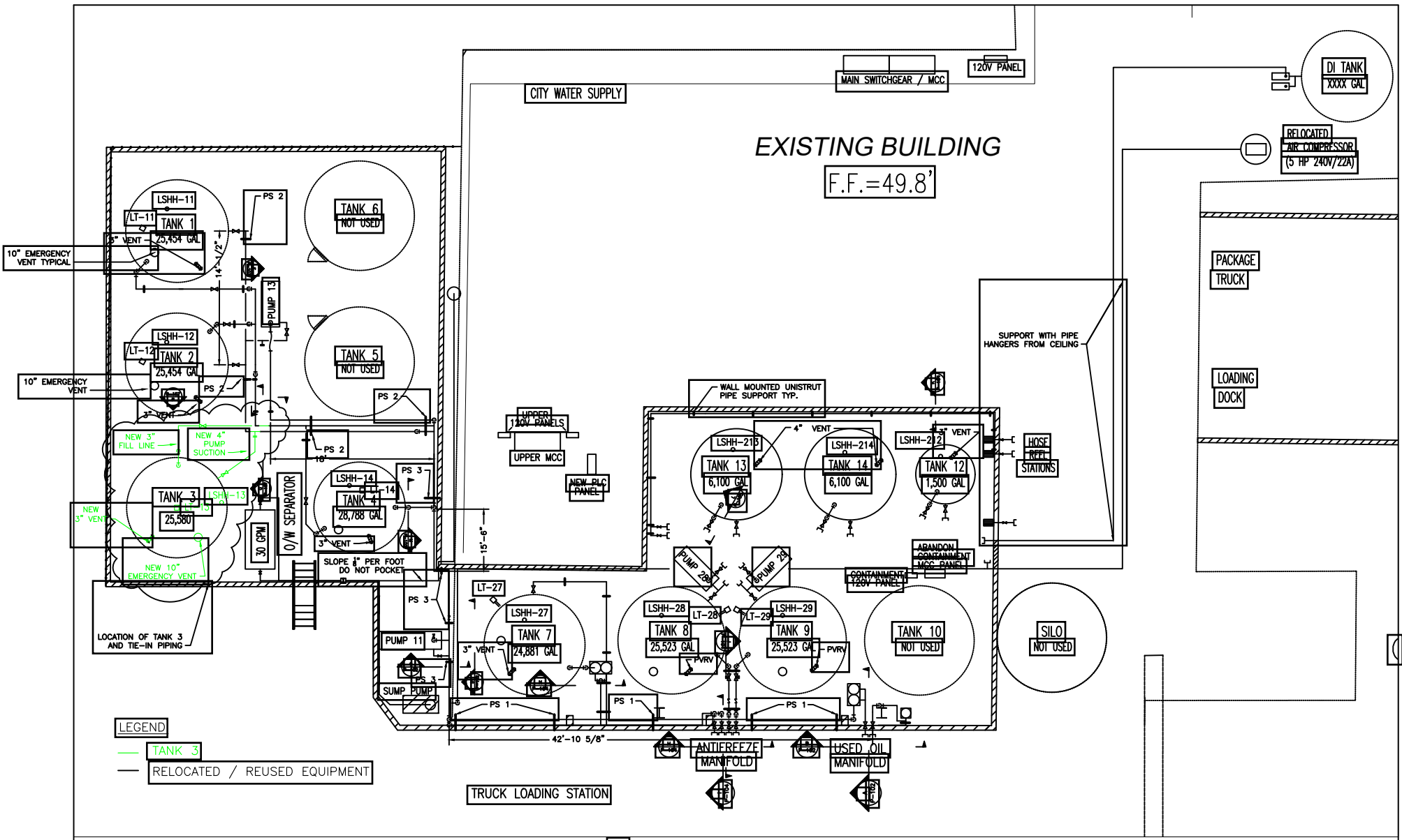
PIPING PLAN NOT TO SCALE
